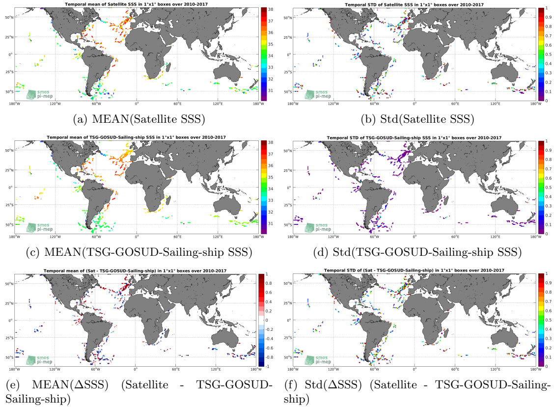
Figure 6: Temporal mean (left) and Std (right) of SSS from SMOS L2 v662 (ESA) (top), TSG-GOSUD-Sailing-ship (middle), and of \Delta SSS (Satellite - TSG-GOSUD-Sailing-ship). Only match-up pairs are used to generate these maps.
