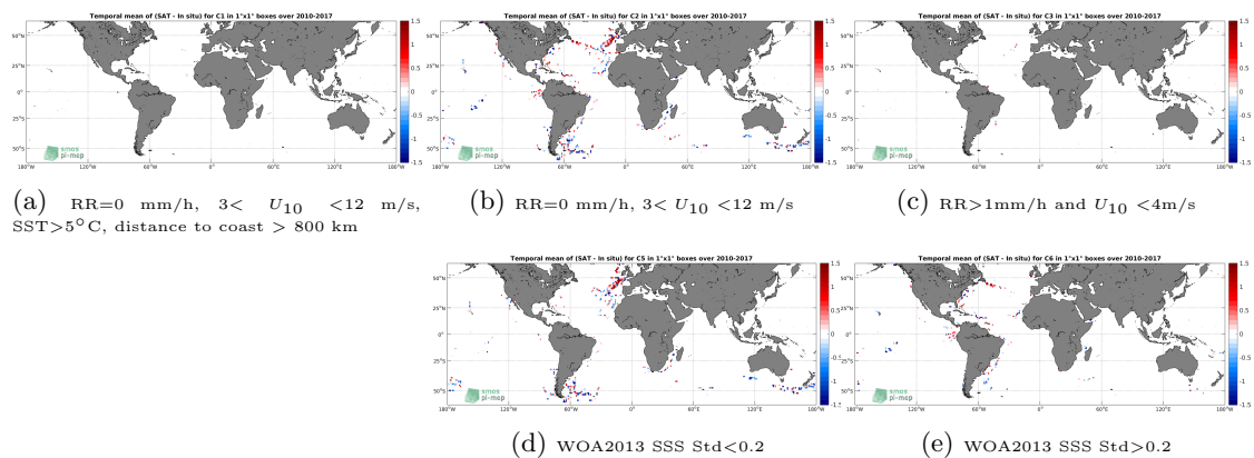
Figure 12: Temporal mean gridded over spatial boxes of size 1^\circ \times 1^\circ of \Delta SSS (SMOS L2 v662 (ESA) - TSG-GOSUD-Sailing-ship) for 5 different subdatasets corresponding to:RR=0 mm/h, 3 < U_{10} < 12 m/s, SST >5^\circ\text{C} , distance to coast > 800 km (a), RR=0 mm/h, 3 < U_{10} < 12 m/s (b), RR >1 mm/h and U_{10} < 4 m/s (c), WOA2013 SSS Std <0.2 (d), WOA2013 SSS Std >0.2 (e).
