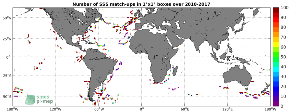
Figure 4: Number of SSS match-ups between TSG-GOSUD-Sailing-ship SSS and the SMOS L2 v662 (ESA) SSS product for the SMOS coastal zone (<800km) 60N-60S Pi-MEP region over 1^\circ \times 1^\circ boxes and for the full satellite product period.
