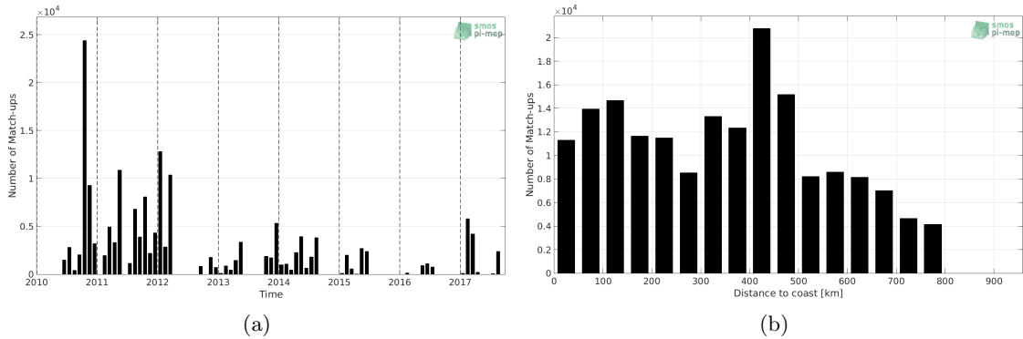
Figure 1: Number of match-ups between TSG-GOSUD-Sailing-ship and SMOS L2 v662 (ESA) SSS as a function of time (a) and as function of the distance to coast (b) over the SMOS coastal zone (<800km) 60N-60S Pi-MEP region and for the full satellite product period.
