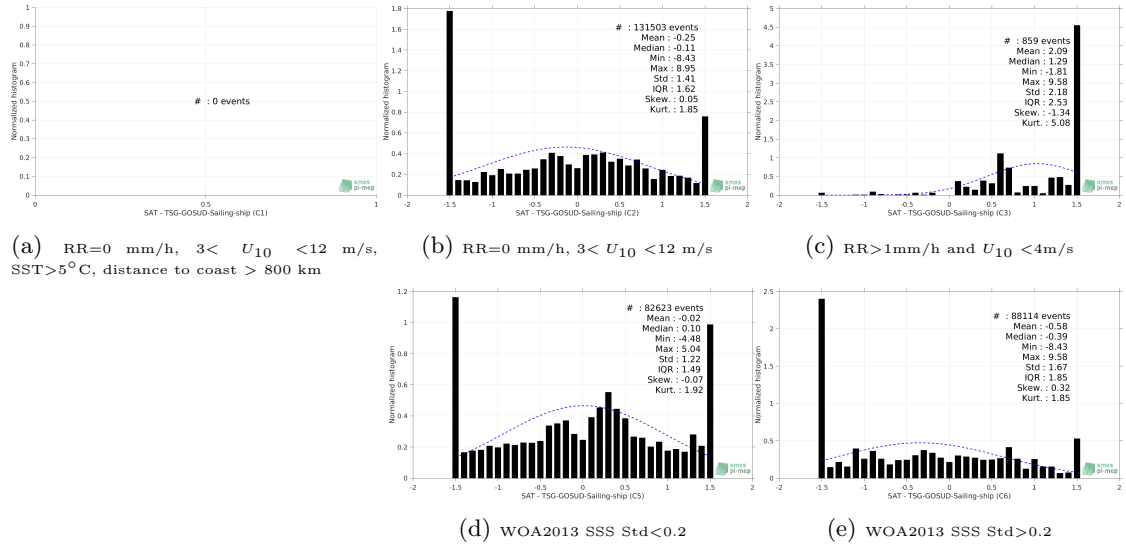
Figure 13: Normalized histogram of \Delta SSS (SMOS L2 v662 (ESA) - TSG-GOSUD-Sailing-ship) for 5 different subdatasets corresponding to: RR=0 mm/h, 3 < U_{10} < 12 m/s, SST > 5°C, distance to coast > 800 km (a), RR=0 mm/h, 3 < U_{10} < 12 m/s (b), RR > 1mm/h and U_{10} < 4 m/s (c), WOA2013 SSS Std < 0.2 (d), WOA2013 SSS Std > 0.2 (e).
