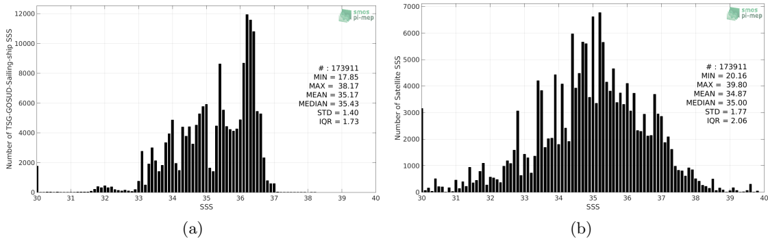
Figure 2: Histograms of SSS from TSG-GOSUD-Sailing-ship (a) and SMOS L2 v662 (ESA) (b) considering all match-up pairs per bins of 0.1 over the SMOS coastal zone (<800km) 60N-60S Pi-MEP region and for the full satellite product period.
