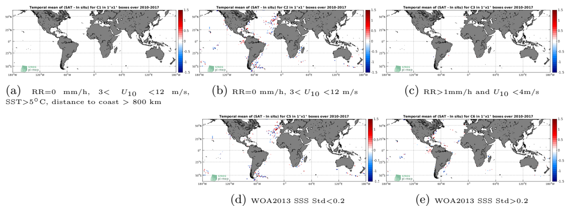
Figure 12: Temporal mean gridded over spatial boxes of size 1^\circ \times 1^\circ of \Delta SSS (SMOS-L2-DPGS-v662 - TSG-GOSUD-Sailing-ship) for 5 different subdatasets corresponding to: RR=0 mm/h, 3 < U_{10} < 12 m/s, SST > 5°C, distance to coast > 800 km (a), RR=0 mm/h, 3 < U_{10} < 12 m/s (b), RR > 1mm/h and U_{10} < 4 m/s (c), WOA2013 SSS Std < 0.2 (d), WOA2013 SSS Std > 0.2 (e).
