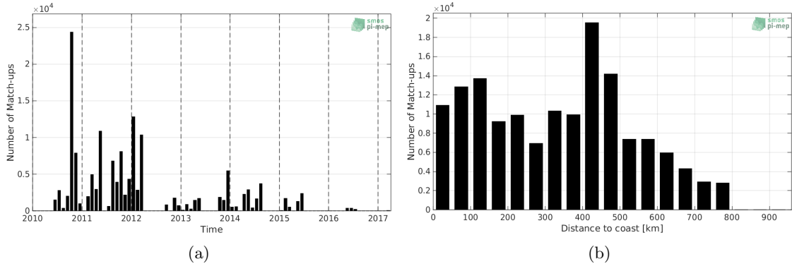
Figure 1: Number of match-ups between TSG-GOSUD-Sailing-ship and SMOS-L2-DPGS-v662 SSS as a function of time (a) and as function of the distance to coast (b) over the SMOS coastal zone ( \approx 800 km) 60N-60S Pi-MEP region and for the full satellite product period.
