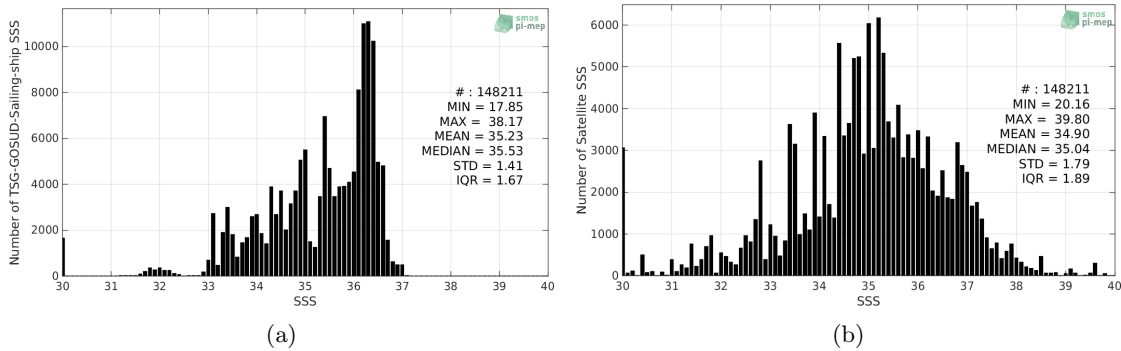
Figure 2: Histograms of SSS from TSG-GOSUD-Sailing-ship (a) and SMOS-L2-DPGS-v662 (b) considering all match-up pairs per bins of 0.1 over the SMOS coastal zone ( \approx 800 km) 60N-60S Pi-MEP region and for the full satellite product period.
