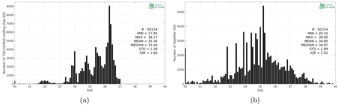
Figure 2: Histograms of SSS from TSG-GOSUD-Sailing-ship (a) and SMOS-L2-DPGS-v662 (b) considering all match-up pairs per bins of 0.1 over the SMOS coastal zone ( \approx 800\text{km} ) 60N-60S Pi-MEP region and for the full satellite product period.
