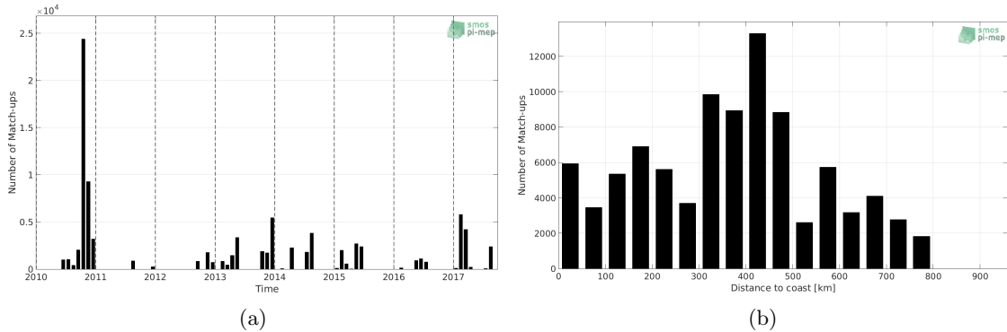
Figure 1: Number of match-ups between TSG-GOSUD-Sailing-ship and SMOS-L2-DPGS-v662 SSS as a function of time (a) and as function of the distance to coast (b) over the SMOS coastal zone ( \approx 800\text{km} ) 60N-60S Pi-MEP region and for the full satellite product period.
