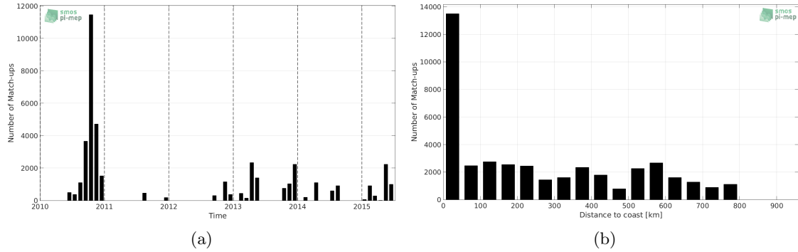
Figure 1: Number of match-ups between TSG-GOSUD-Sailing-ship and SMOS-L2-DPGS-v662 SSS as a function of time (a) and as function of the distance to coast (b) over the SMOS coastal zone ( \geq 800\text{km} ) 60N-60S Pi-MEP region and for the full satellite product period.
