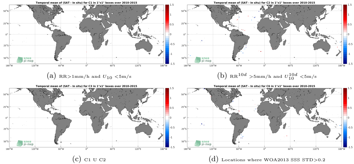
Figure 12: Temporal mean gridded over spatial boxes of size 1^\circ \times 1^\circ of \Delta SSS (SMOS-L2-DPGS-v662 - TSG-GOSUD-Sailing-ship) for 4 different subdatasets corresponding to: RR > 1\text{mm/h} and U_{10} < 5\text{m/s} (a), RR^{10d} > 5\text{mm/h} and U_{10}^{10d} < 5\text{m/s} (b), C1 U C2 (c), Locations where WOA2013 SSS STD > 0.2 (d).
