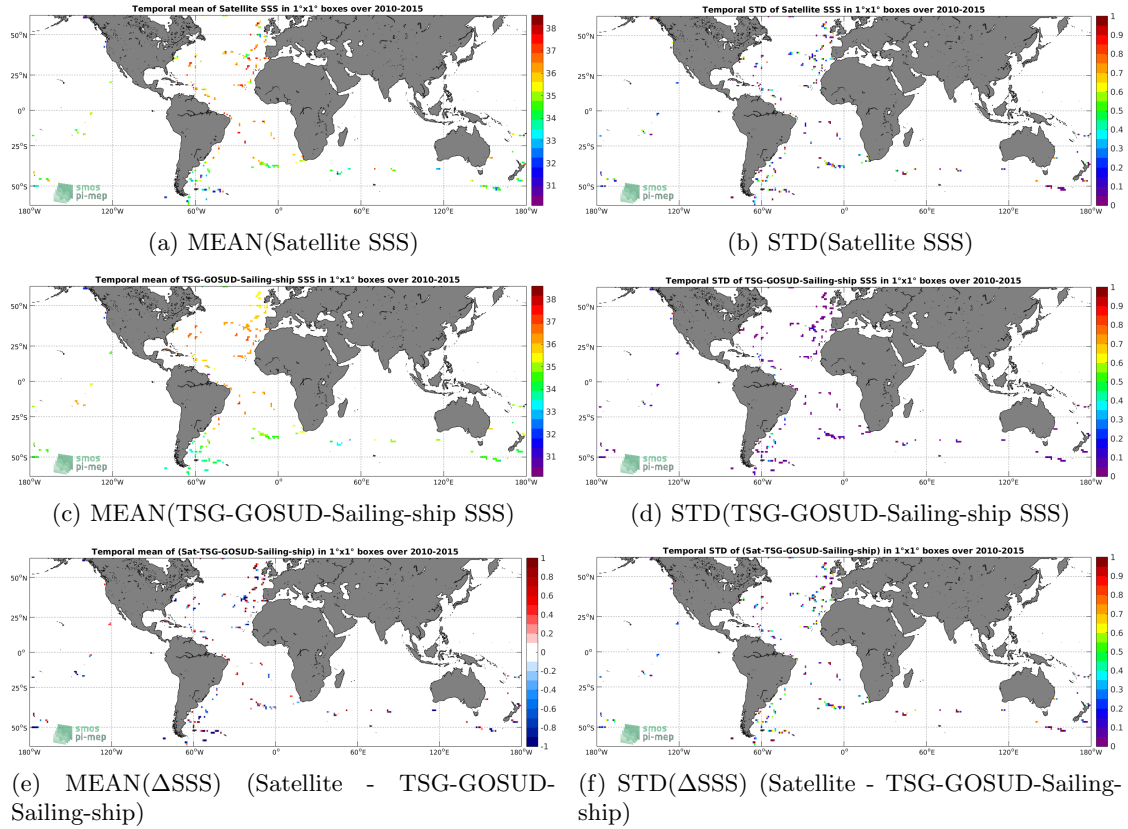
Figure 6: Temporal mean (left) and STD (right) of SSS from SMOS-L2-DPGS-v662 (top), TSG-GOSUD-Sailing-ship (middle), and of \Delta SSS (Satellite - TSG-GOSUD-Sailing-ship). Only match-up pairs are used to generate these maps.
