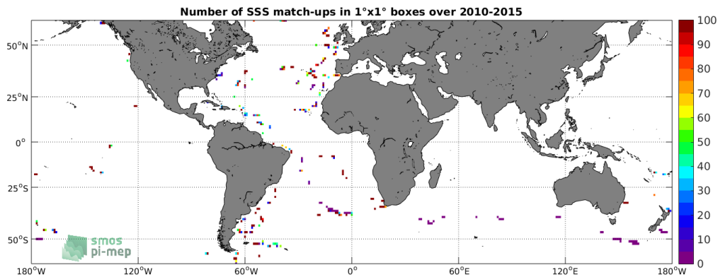
Figure 4: Number of SSS match-ups between TSG-GOSUD-Sailing-ship SSS and the SMOS-L2-DPGS-v662 SSS product for the SMOS coastal zone ( \pm 800\text{km} ) 60N-60S Pi-MEP region over 1^\circ \times 1^\circ boxes and for the full satellite product period.
