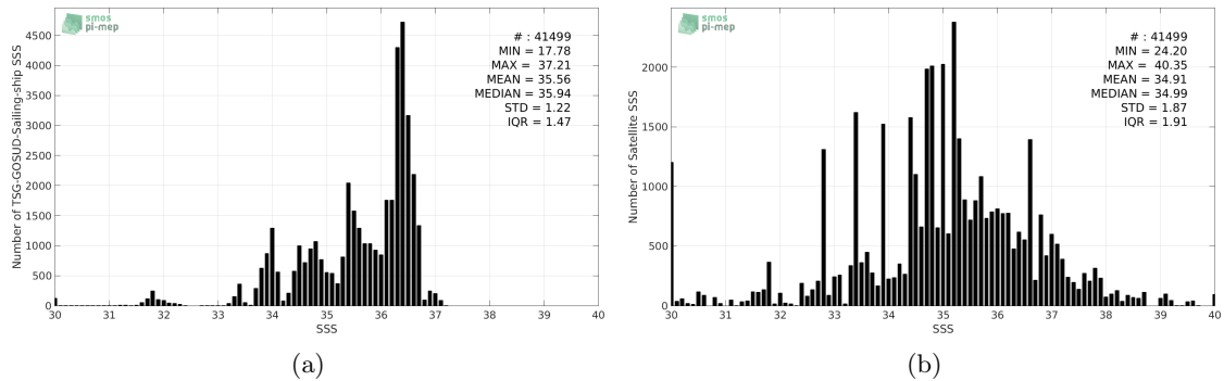
Figure 2: Histograms of SSS from TSG-GOSUD-Sailing-ship (a) and SMOS-L2-DPGS-v662 (b) considering all match-up pairs per bins of 0.1 over the SMOS coastal zone ( \geq 800\text{km} ) 60N-60S Pi-MEP region and for the full satellite product period.
