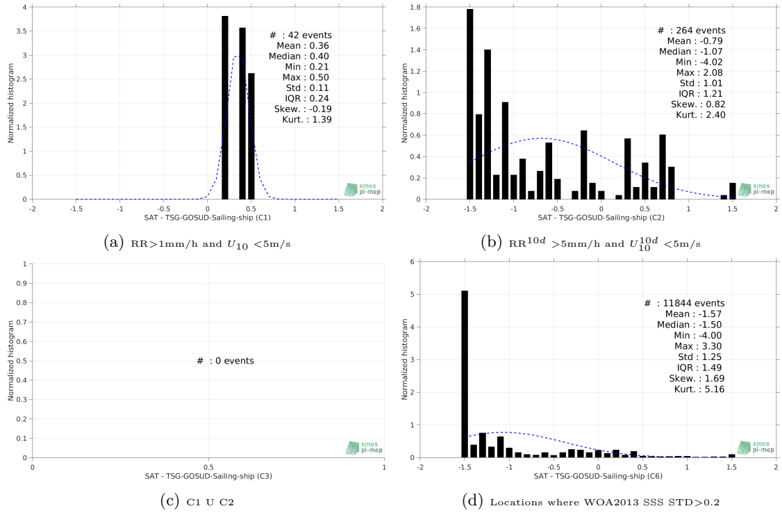
Figure 13: Normalized histogram of \Delta\text{SSS} (SMOS-L2-DPGS-v662 - TSG-GOSUD-Sailing-ship) for 6 different subdatasets corresponding to: RR > 1\text{mm/h} and U_{10} < 5\text{m/s} (a), RR^{10d} > 5\text{mm/h} and U_{10}^{10d} < 5\text{m/s} (b), C1 U C2 (c), Locations where WOA2013 SSS STD > 0.2 (d).
