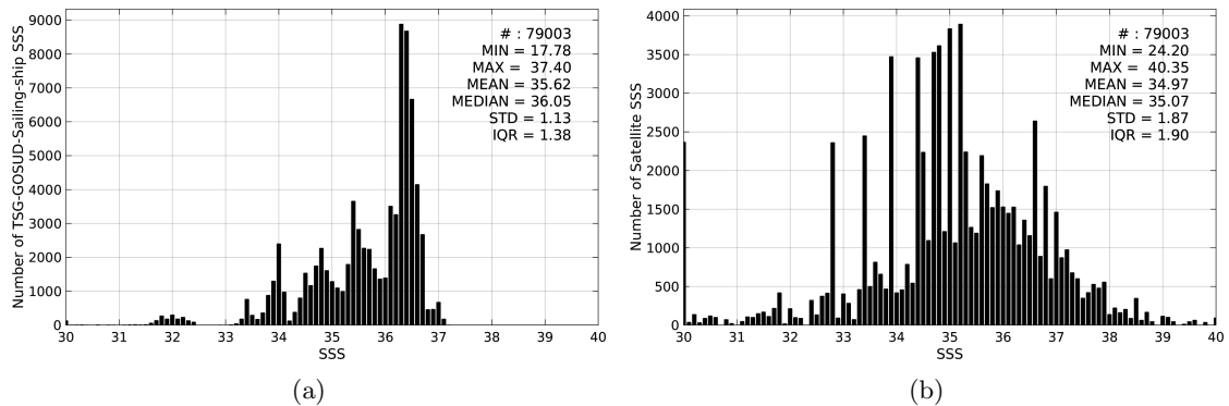
Figure 2: Histograms of SSS from TSG-GOSUD-Sailing-ship (a) and SMOS-L2-DPGS-v662 (b) considering all match-up pairs per bins of 0.1 over the SMOS coastal zone ( \geq 800 km) 60N-60S Pi-MEP region and for the full satellite product period.
