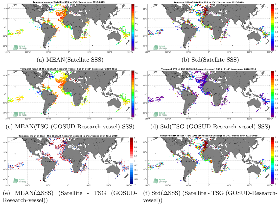
Figure 6: Temporal mean (left) and Std (right) of SSS from SMOS SSS L2 v662 (ESA) (top), TSG (GOSUD-Research-vessel) (middle), and of \Delta SSS (Satellite - TSG (GOSUD-Research-vessel)). Only match-up pairs are used to generate these maps.
