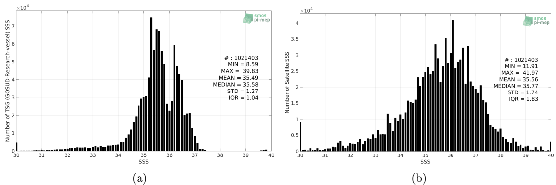
Figure 2: Histograms of SSS from TSG (GOSUD-Research-vessel) (a) and SMOS SSS L2 v662 (ESA) (b) considering all match-up pairs per bins of 0.1 over the SMOS coastal zone (<800km) 60N-60S Pi-MEP region and for the full satellite product period.
