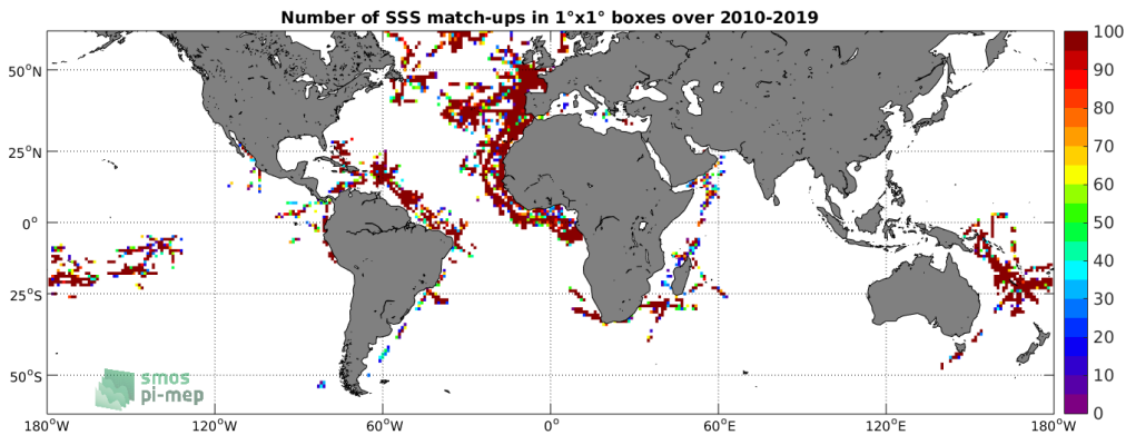
Figure 4: Number of SSS match-ups between TSG (GOSUD-Research-vessel) SSS and the SMOS SSS L2 v662 (ESA) SSS product for the SMOS coastal zone (<800km) 60N-60S Pi-MEP region over 1°x1° boxes and for the full satellite product period.
