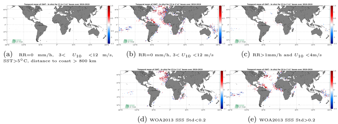
Figure 12: Temporal mean gridded over spatial boxes of size 1^\circ \times 1^\circ of \Delta SSS (SMOS SSS L2 v662 (ESA) - TSG (GOSUD-Research-vessel)) for 5 different subdatasets corresponding to:RR=0 mm/h, 3 < U_{10} < 12 m/s, SST > 5°C, distance to coast > 800 km (a), RR=0 mm/h, 3 < U_{10} < 12 m/s (b), RR > 1mm/h and U_{10} < 4 m/s (c), WOA2013 SSS Std < 0.2 (d), WOA2013 SSS Std > 0.2 (e).
