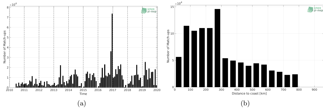
Figure 1: Number of match-ups between TSG (GOSUD-Research-vessel) and SMOS SSS L2 v662 (ESA) SSS as a function of time (a) and as function of the distance to coast (b) over the SMOS coastal zone (<800km) 60N-60S Pi-MEP region and for the full satellite product period.
