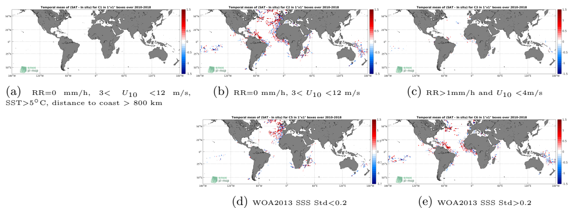
Figure 12: Temporal mean gridded over spatial boxes of size 1^\circ \times 1^\circ of \Delta SSS (SMOS L2 v662 (ESA) - TSG-GOSUD-Research-vessel) for 5 different subdatasets corresponding to:RR=0 mm/h, 3 < U_{10} < 12 m/s, SST >5^\circ\text{C} , distance to coast > 800 km (a), RR=0 mm/h, 3 < U_{10} < 12 m/s (b), RR >1 mm/h and U_{10} < 4 m/s (c), WOA2013 SSS Std <0.2 (d), WOA2013 SSS Std >0.2 (e).
