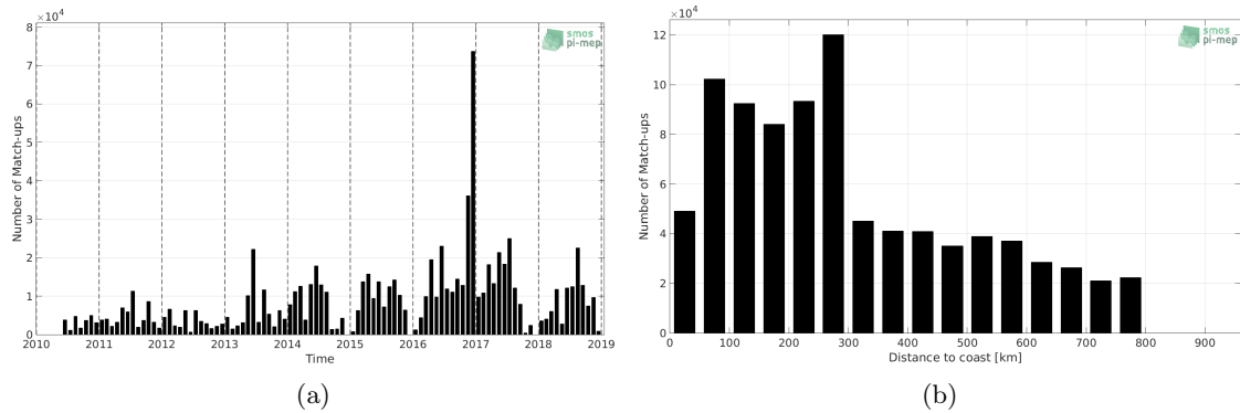
Figure 1: Number of match-ups between TSG-GOSUD-Research-vessel and SMOS L2 v662 (ESA) SSS as a function of time (a) and as function of the distance to coast (b) over the SMOS coastal zone (<800km) 60N-60S Pi-MEP region and for the full satellite product period.
