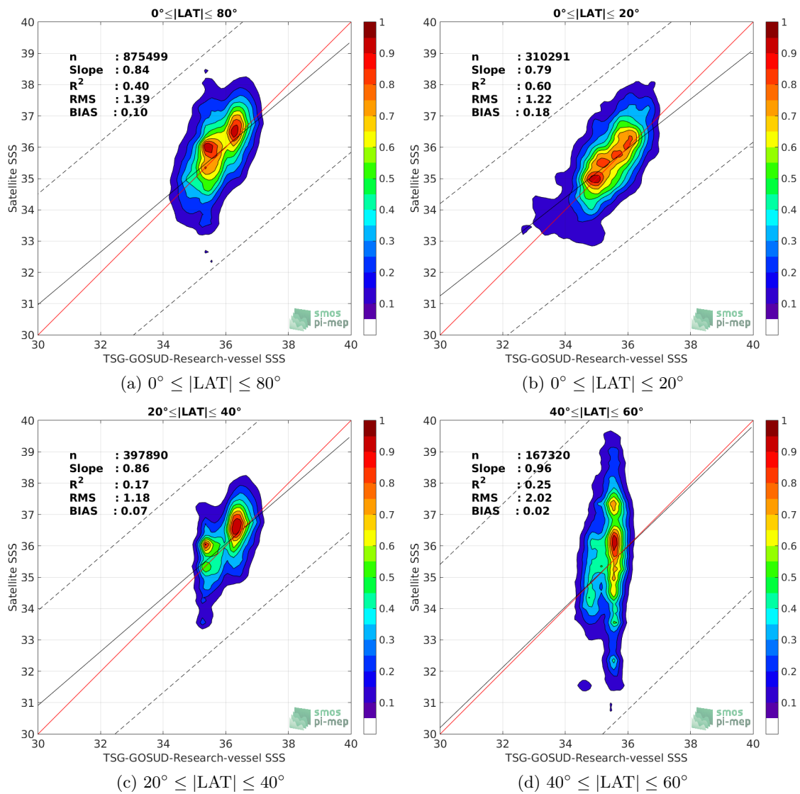
Figure 9: Contour maps of the concentration of SMOS L2 v662 (ESA) SSS ( y -axis) versus TSG-GOSUD-Research-vessel SSS ( x -axis) at match-up pairs for different latitude bands. For each plot, the red line shows x=y . The black thin and dashed lines indicate a linear fit through the data cloud and the \pm 95\% confidence levels, respectively. The number match-up pairs n , the slope and R^2 coefficient of the linear fit, the root mean square (RMS) and the mean bias between satellite and in situ data are indicated for each latitude band in each plots.
