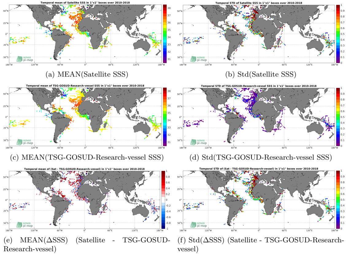
Figure 6: Temporal mean (left) and Std (right) of SSS from SMOS L2 v662 (ESA) (top), TSG-GOSUD-Research-vessel (middle), and of \Delta SSS (Satellite - TSG-GOSUD-Research-vessel). Only match-up pairs are used to generate these maps.
