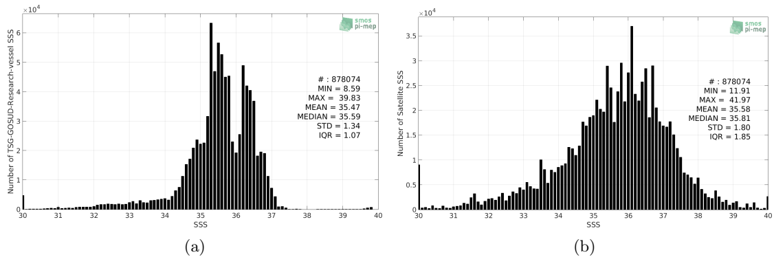
Figure 2: Histograms of SSS from TSG-GOSUD-Research-vessel (a) and SMOS L2 v662 (ESA) (b) considering all match-up pairs per bins of 0.1 over the SMOS coastal zone (<800km) 60N-60S Pi-MEP region and for the full satellite product period.
