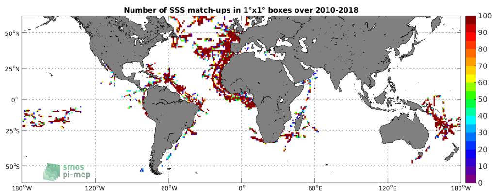
Figure 4: Number of SSS match-ups between TSG-GOSUD-Research-vessel SSS and the SMOS L2 v662 (ESA) SSS product for the SMOS coastal zone (<800km) 60N-60S Pi-MEP region over 1^\circ \times 1^\circ boxes and for the full satellite product period.
