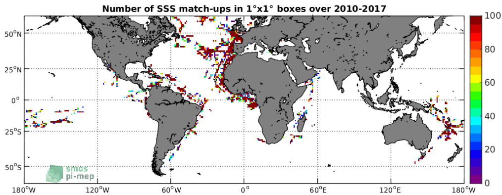
Figure 4: Number of SSS match-ups between TSG-GOSUD-Research-vessel SSS and the SMOS-L2-DPGS-v662 SSS product for the SMOS coastal zone ( \approx 800\text{km} ) 60N-60S Pi-MEP region over 1^\circ \times 1^\circ boxes and for the full satellite product period.
