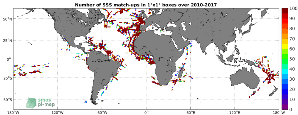
Figure 4: Number of SSS match-ups between TSG-GOSUD-Research-vessel SSS and the SMOS-L2-DPGS-v662 SSS product for the SMOS coastal zone ( \pm 800\text{km} ) 60N-60S Pi-MEP region over 1^\circ \times 1^\circ boxes and for the full satellite product period.
