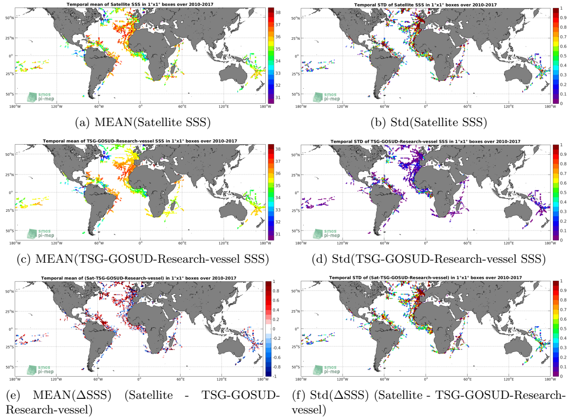
Figure 6: Temporal mean (left) and Std (right) of SSS from SMOS-L2-DPGS-v662 (top), TSG-GOSUD-Research-vessel (middle), and of \Delta SSS (Satellite - TSG-GOSUD-Research-vessel). Only match-up pairs are used to generate these maps.
