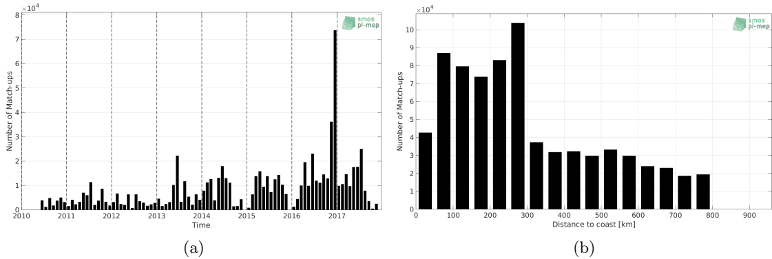
Figure 1: Number of match-ups between TSG-GOSUD-Research-vessel and SMOS-L2-DPGS-v662 SSS as a function of time (a) and as function of the distance to coast (b) over the SMOS coastal zone ( \approx 800 km) 60N-60S Pi-MEP region and for the full satellite product period.
