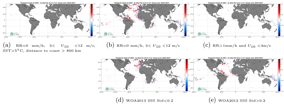
Figure 12: Temporal mean gridded over spatial boxes of size 1^\circ \times 1^\circ of \Delta SSS (SMOS-L2-DPGS-v662 - TSG-GOSUD-Research-vessel) for 5 different subdatasets corresponding to:RR=0 mm/h, 3 < U_{10} < 12 m/s, SST >5^\circ C, distance to coast > 800 km (a), RR=0 mm/h, 3 < U_{10} < 12 m/s (b), RR >1 mm/h and U_{10} < 4 m/s (c), WOA2013 SSS Std <0.2 (d), WOA2013 SSS Std >0.2 (e).
