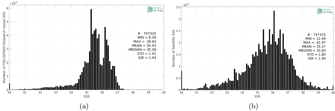
Figure 2: Histograms of SSS from TSG-GOSUD-Research-vessel (a) and SMOS-L2-DPGS-v662 (b) considering all match-up pairs per bins of 0.1 over the SMOS coastal zone ( \approx 800 km) 60N-60S Pi-MEP region and for the full satellite product period.
