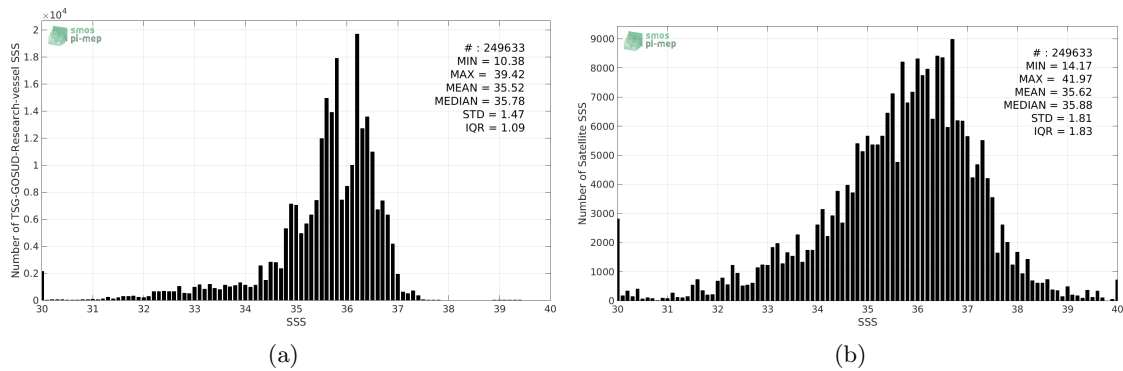
Figure 2: Histograms of SSS from TSG-GOSUD-Research-vessel (a) and SMOS-L2-DPGS-v662 (b) considering all match-up pairs per bins of 0.1 over the SMOS coastal zone ( \approx 800\text{km} ) 60N-60S Pi-MEP region and for the full satellite product period.
