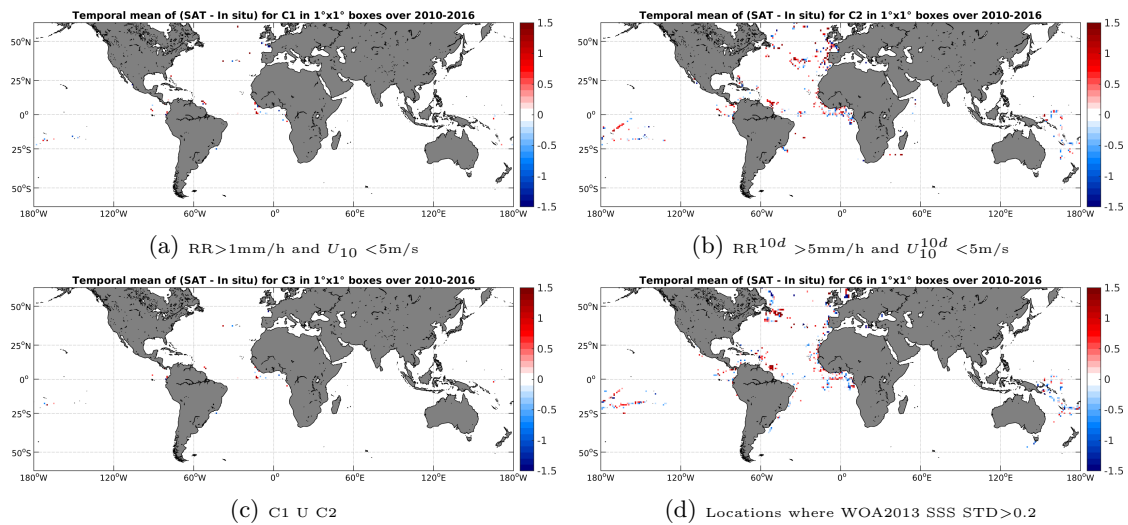
Figure 12: Temporal mean gridded over spatial boxes of size 1^\circ \times 1^\circ of \Delta SSS (SMOS-L2-DPGS-v662 - TSG-GOSUD-Research-vessel) for 4 different subdatasets corresponding to: RR > 1\text{mm/h} and U_{10} < 5\text{m/s} (a), RR^{10d} > 5\text{mm/h} and U_{10}^{10d} < 5\text{m/s} (b), C1 U C2 (c), Locations where WOA2013 SSS STD > 0.2 (d).
