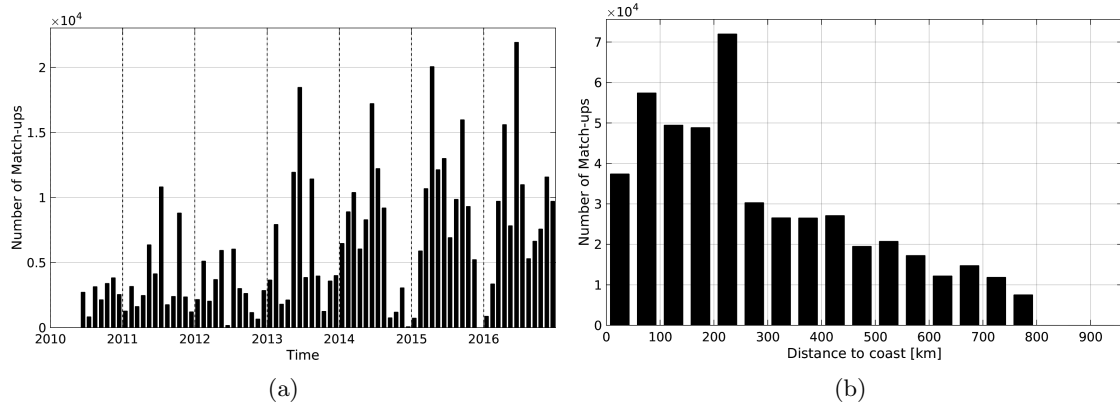
Figure 1: Number of match-ups between TSG-GOSUD-Research-vessel and SMOS-L2-DPGS-v662 SSS as a function of time (a) and as function of the distance to coast (b) over the SMOS coastal zone ( \approx 800 km) 60N-60S Pi-MEP region and for the full satellite product period.
