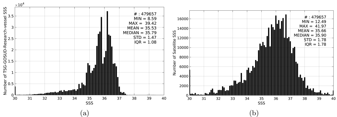
Figure 2: Histograms of SSS from TSG-GOSUD-Research-vessel (a) and SMOS-L2-DPGS-v662 (b) considering all match-up pairs per bins of 0.1 over the SMOS coastal zone ( \approx 800 km) 60N-60S Pi-MEP region and for the full satellite product period.
