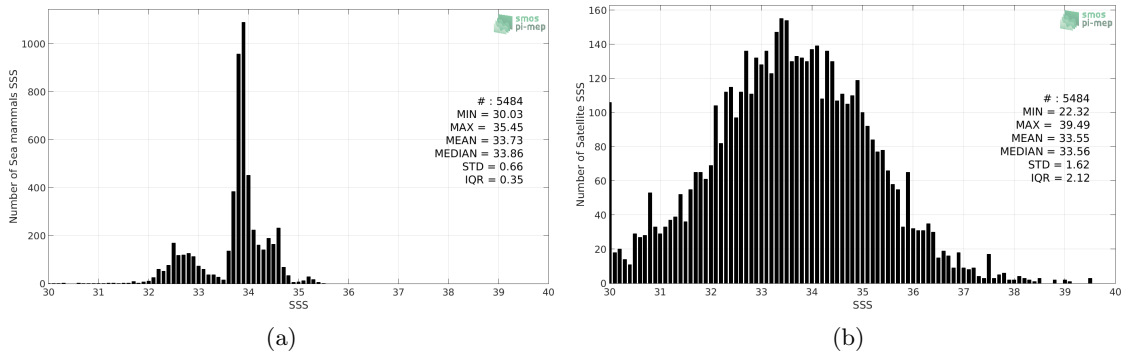
Figure 2: Histograms of SSS from Sea mammals (a) and SMOS SSS L2 v662 (ESA) (b) considering all match-up pairs per bins of 0.1 over the SMOS coastal zone (<800km) 60N-60S Pi-MEP region and for the full satellite product period.
