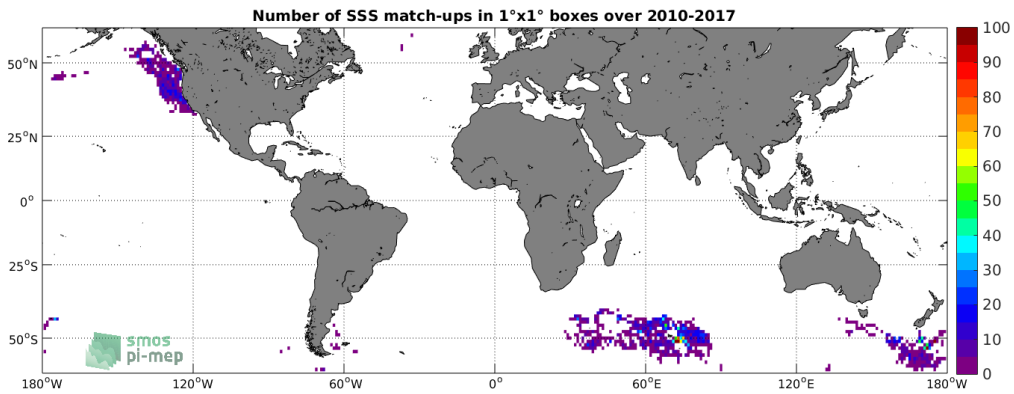
Figure 4: Number of SSS match-ups between Sea mammals SSS and the SMOS SSS L2 v662 (ESA) SSS product for the SMOS coastal zone (<800km) 60N-60S Pi-MEP region over 1°x1° boxes and for the full satellite product period.
