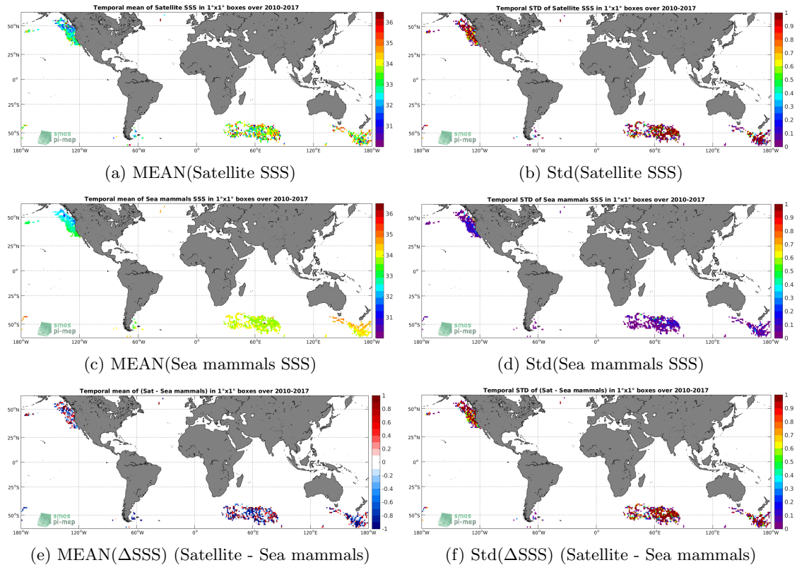
Figure 6: Temporal mean (left) and Std (right) of SSS from SMOS SSS L2 v662 (ESA) (top), Sea mammals (middle), and of \Delta SSS (Satellite - Sea mammals). Only match-up pairs are used to generate these maps.
