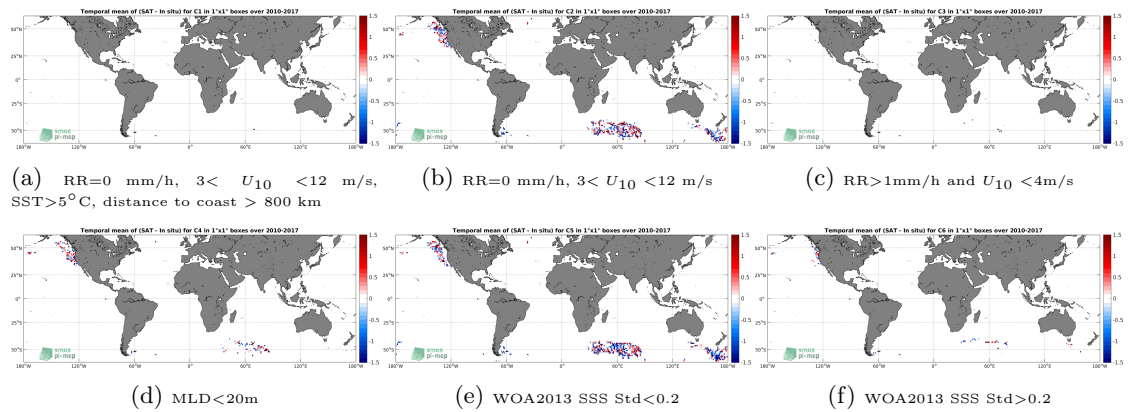
Figure 12: Temporal mean gridded over spatial boxes of size 1°x1° of \Delta SSS (SMOS SSS L2 v662 (ESA) - Sea mammals) for 6 different subdatasets corresponding to:RR=0 mm/h, 3 < U_{10} < 12 m/s, SST>5°C, distance to coast > 800 km (a), RR=0 mm/h, 3 < U_{10} < 12 m/s (b), RR>1mm/h and U_{10} < 4 m/s (c),MLD<20m (d),WOA2013 SSS Std<0.2 (e),WOA2013 SSS Std>0.2 (f).
