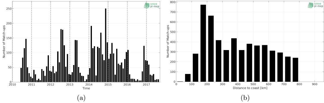
Figure 1: Number of match-ups between Sea mammals and SMOS SSS L2 v662 (ESA) SSS as a function of time (a) and as function of the distance to coast (b) over the SMOS coastal zone (<800km) 60N-60S Pi-MEP region and for the full satellite product period.
