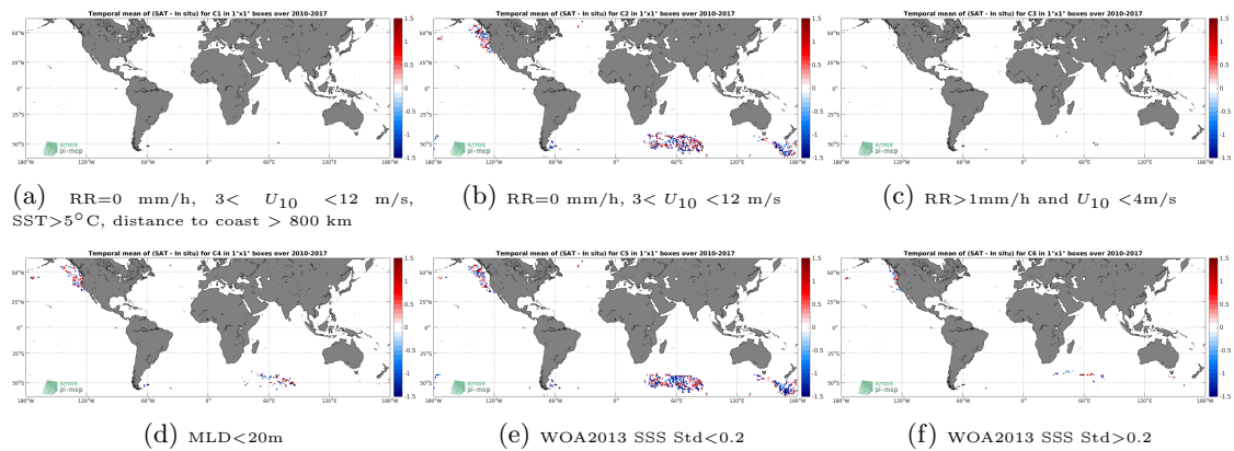
Figure 12: Temporal mean gridded over spatial boxes of size 1^\circ \times 1^\circ of \Delta SSS (SMOS L2 v662 (ESA) - Sea mammals) for 6 different subdatasets corresponding to:RR=0 mm/h, 3 < U_{10} < 12 m/s, SST >5^\circ C, distance to coast > 800 km (a), RR=0 mm/h, 3 < U_{10} < 12 m/s (b), RR >1 mm/h and U_{10} < 4 m/s (c),MLD <20 m (d),WOA2013 SSS Std <0.2 (e),WOA2013 SSS Std >0.2 (f).
