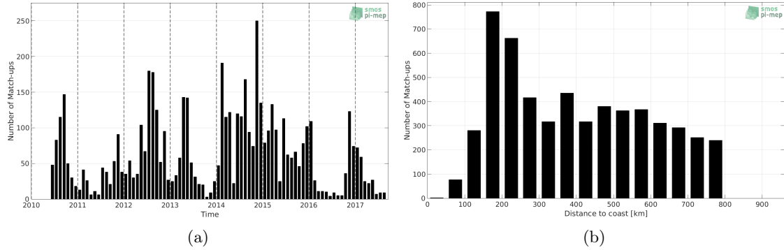
Figure 1: Number of match-ups between Sea mammals and SMOS L2 v662 (ESA) SSS as a function of time (a) and as function of the distance to coast (b) over the SMOS coastal zone (<800km) 60N-60S Pi-MEP region and for the full satellite product period.
