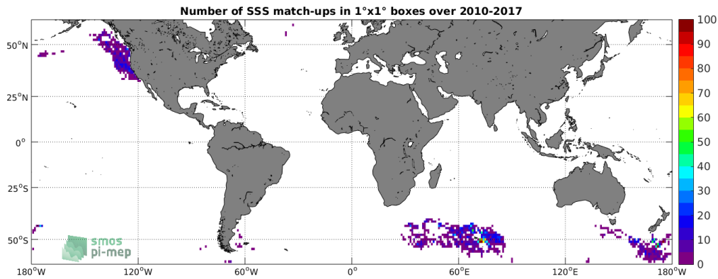
Figure 4: Number of SSS match-ups between Sea mammals SSS and the SMOS L2 v662 (ESA) SSS product for the SMOS coastal zone (<800km) 60N-60S Pi-MEP region over 1°x1° boxes and for the full satellite product period.
