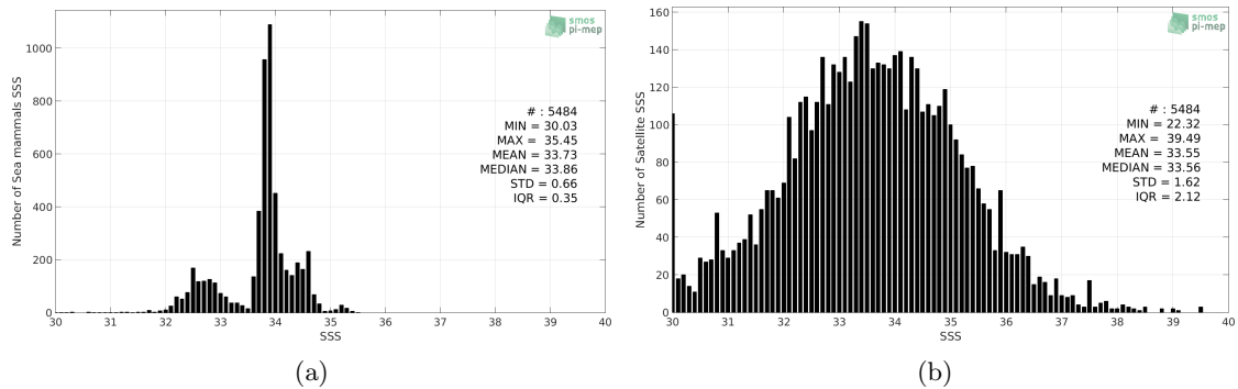
Figure 2: Histograms of SSS from Sea mammals (a) and SMOS L2 v662 (ESA) (b) considering all match-up pairs per bins of 0.1 over the SMOS coastal zone (<800km) 60N-60S Pi-MEP region and for the full satellite product period.
