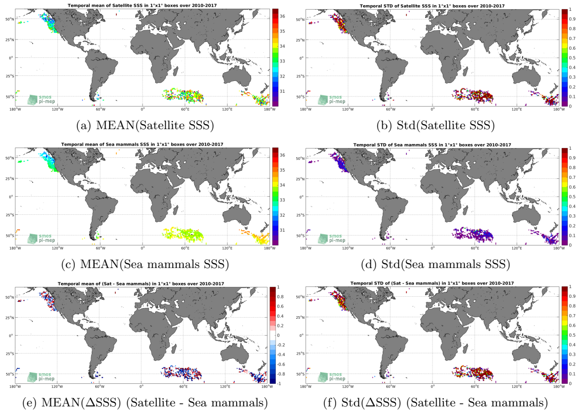
Figure 6: Temporal mean (left) and Std (right) of SSS from SMOS L2 v662 (ESA) (top), Sea mammals (middle), and of \Delta SSS (Satellite - Sea mammals). Only match-up pairs are used to generate these maps.
