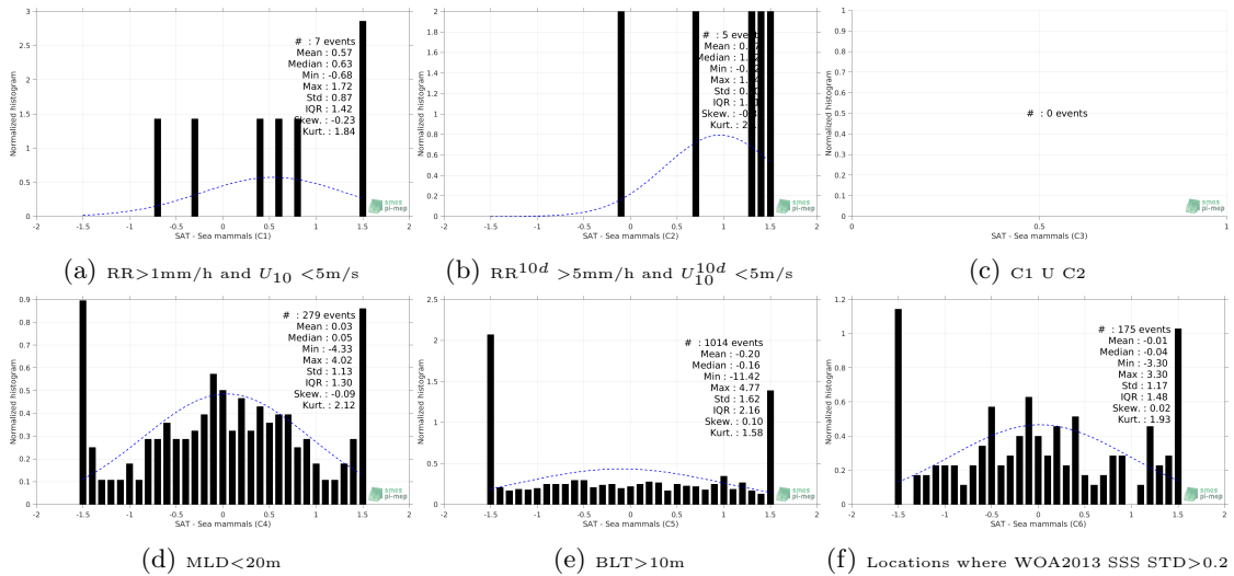
Figure 13: Normalized histogram of \Delta SSS (SMOS-L2-DPGS-v662 - Sea mammals) for 6 different subdatasets corresponding to: RR>1mm/h and U_{10} < 5m/s (a), RR^{10d} > 5mm/h and U_{10}^{10d} < 5m/s (b), C1 U C2 (c),MLD<20m (d),BLT>10m (e),Locations where WOA2013 SSS STD>0.2 (f).
