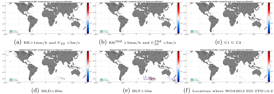
Figure 12: Temporal mean gridded over spatial boxes of size 1^\circ \times 1^\circ of \Delta SSS (SMOS-L2-DPGS-v662 - Sea mammals) for 6 different subdatasets corresponding to:RR>1mm/h and U_{10} < 5m/s (a), RR^{10d} > 5mm/h and U_{10}^{10d} < 5m/s (b), C1 U C2 (c),MLD<20m (d),BLT>10m (e),Locations where WOA2013 SSS STD>0.2 (f).
