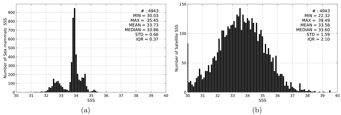
Figure 2: Histograms of SSS from Sea mammals (a) and SMOS-L2-DPGS-v662 (b) considering all match-up pairs per bins of 0.1 over the SMOS coastal zone ( \pm 800\text{km} ) 60N-60S Pi-MEP region and for the full satellite product period.
