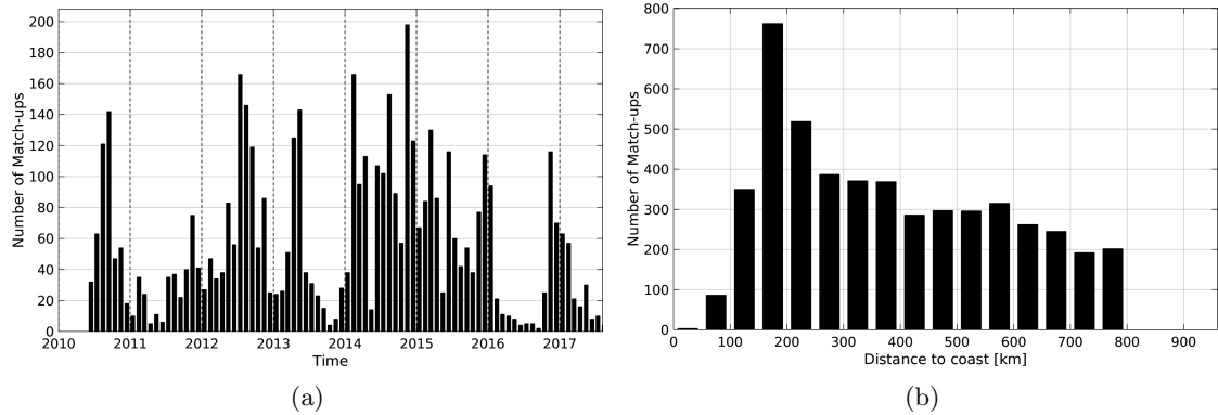
Figure 1: Number of match-ups between Sea mammals and SMOS-L2-DPGS-v662 SSS as a function of time (a) and as function of the distance to coast (b) over the SMOS coastal zone ( \pm 800\text{km} ) 60N-60S Pi-MEP region and for the full satellite product period.
