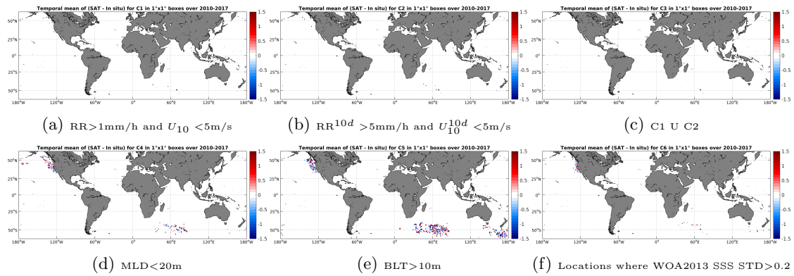
Figure 12: Temporal mean gridded over spatial boxes of size 1^\circ \times 1^\circ of \Delta SSS (SMOS-L2-DPGS-v662 - Sea mammals) for 6 different subdatasets corresponding to: RR > 1\text{mm/h} and U_{10} < 5\text{m/s} (a), RR^{10d} > 5\text{mm/h} and U_{10}^{10d} < 5\text{m/s} (b), C1 \cup C2 (c), MLD < 20\text{m} (d), BLT > 10\text{m} (e), Locations where WOA2013 SSS STD > 0.2 (f).
