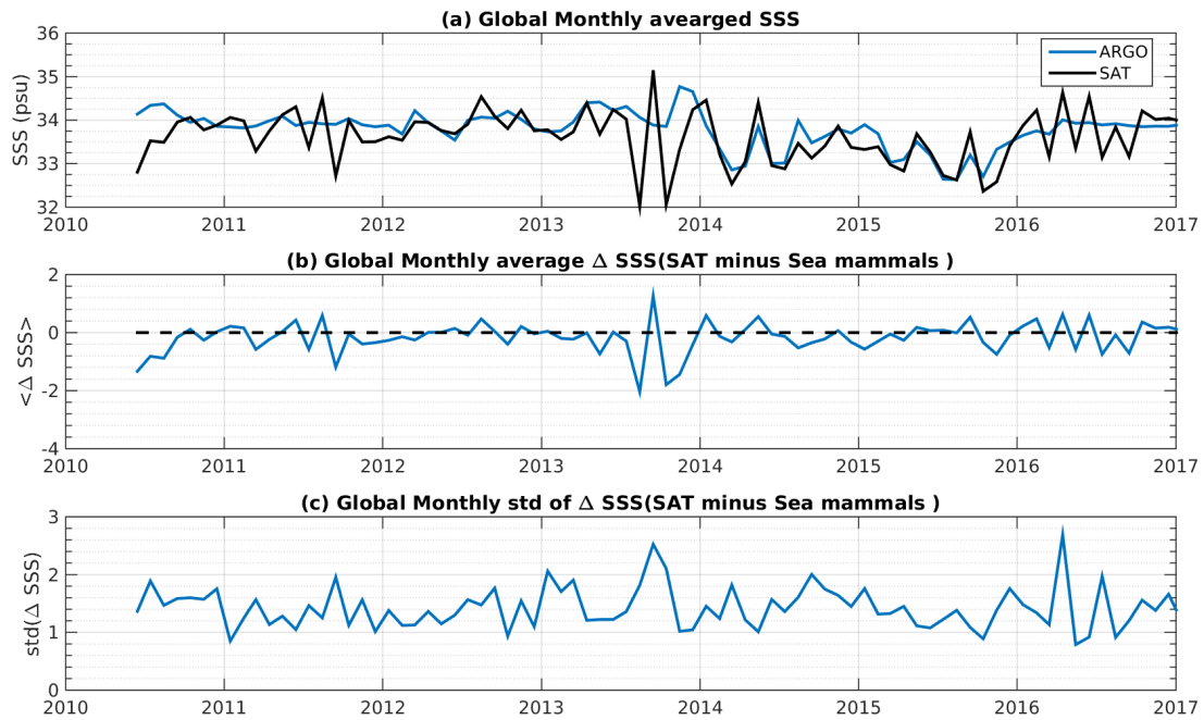
Figure 7: Time series of the monthly averaged mean SSS (top), mean \Delta SSS (Satellite - Sea mammals) and STD of \Delta SSS (Satellite - Sea mammals) over the SMOS coastal zone ( \approx 800 km) 60N-60S Pi-MEP region considering all match-ups collected by the Pi-MEP platform.
