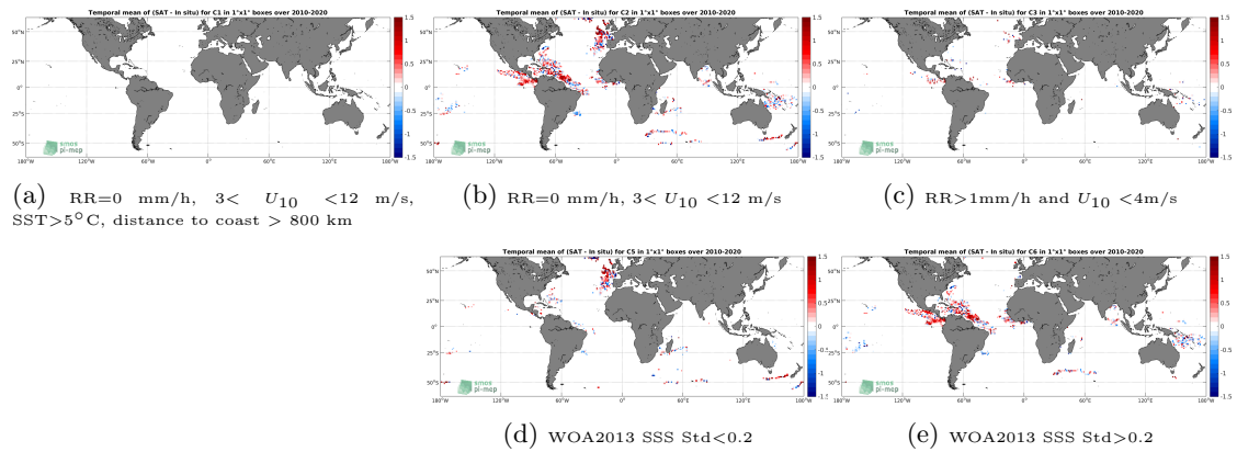
Figure 11: Temporal mean gridded over spatial boxes of size 1^\circ \times 1^\circ of \Delta SSS (SMOS SSS L2 v662 (ESA) - Surface drifters) for 5 different subdatasets corresponding to:RR=0 mm/h, 3 < U_{10} < 12 m/s, SST >5^\circ C, distance to coast > 800 km (a), RR=0 mm/h, 3 < U_{10} < 12 m/s (b), RR >1 mm/h and U_{10} < 4 m/s (c), WOA2013 SSS Std <0.2 (d), WOA2013 SSS Std >0.2 (e).
