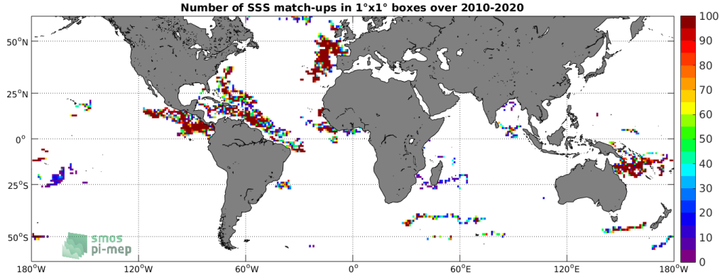
Figure 3: Number of SSS match-ups between Surface drifters SSS and the SMOS SSS L2 v662 (ESA) SSS product for the SMOS coastal zone (<800km) 60N-60S Pi-MEP region over 1^\circ \times 1^\circ boxes and for the full satellite product period.
