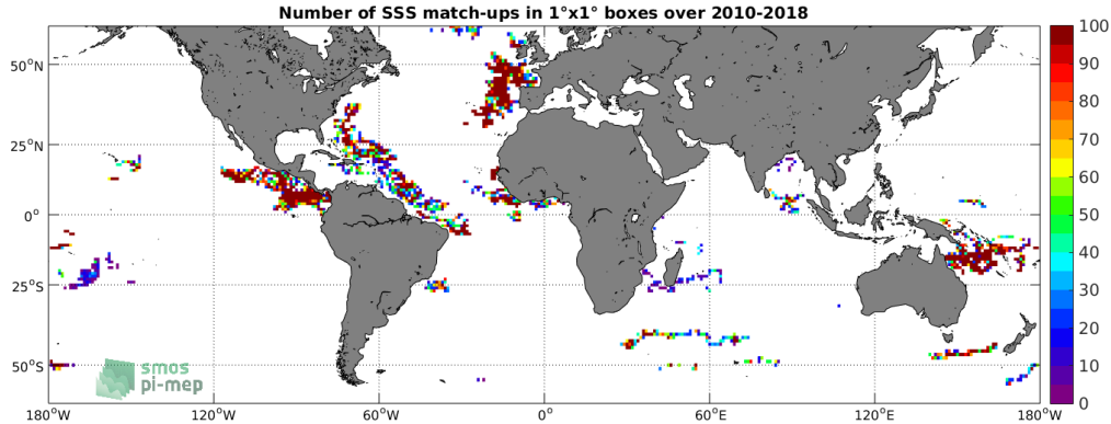
Figure 3: Number of SSS match-ups between Surface drifters SSS and the SMOS L2 v662 (ESA) SSS product for the SMOS coastal zone (<800km) 60N-60S Pi-MEP region over 1^\circ \times 1^\circ boxes and for the full satellite product period.
