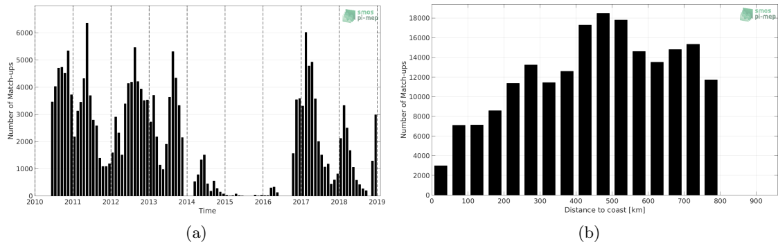
Figure 1: Number of match-ups between Surface drifters and SMOS L2 v662 (ESA) SSS as a function of time (a) and as function of the distance to coast (b) over the SMOS coastal zone (<800km) 60N-60S Pi-MEP region and for the full satellite product period.
