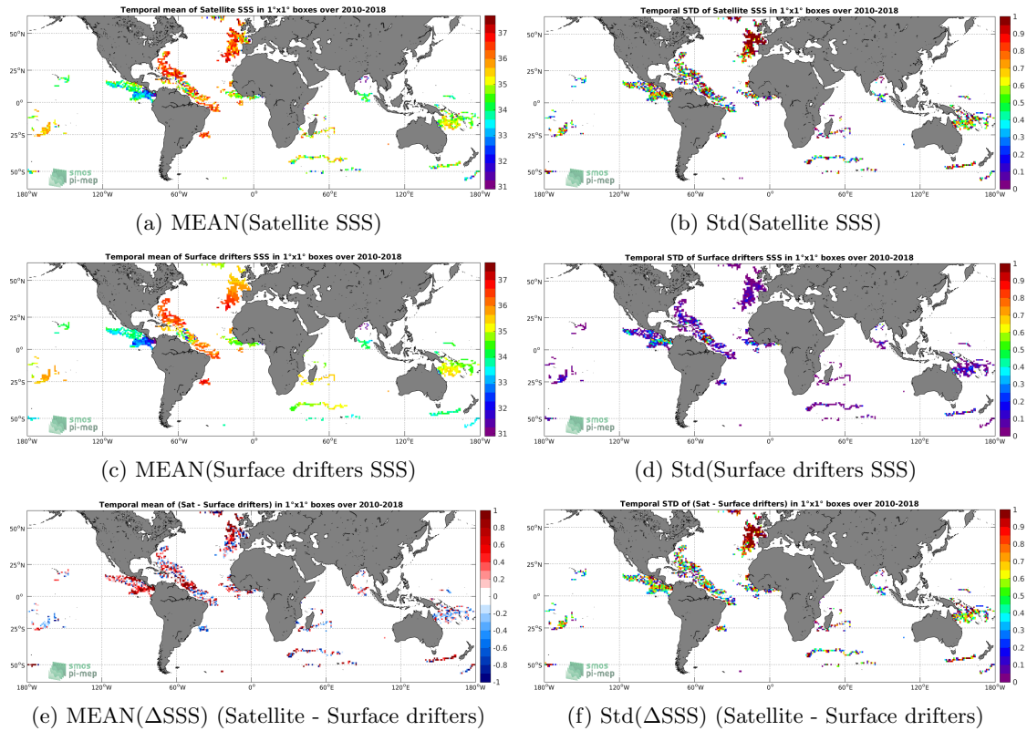
Figure 5: Temporal mean (left) and Std (right) of SSS from SMOS L2 v662 (ESA) (top), Surface drifters (middle), and of \Delta SSS (Satellite - Surface drifters). Only match-up pairs are used to generate these maps.
