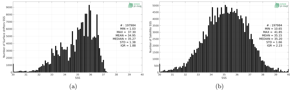
Figure 2: Histograms of SSS from Surface drifters (a) and SMOS L2 v662 (ESA) (b) considering all match-up pairs per bins of 0.1 over the SMOS coastal zone (<800km) 60N-60S Pi-MEP region and for the full satellite product period.
