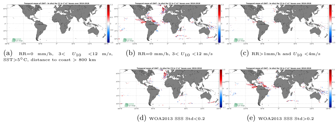
Figure 11: Temporal mean gridded over spatial boxes of size 1^\circ \times 1^\circ of \Delta SSS (SMOS L2 v662 (ESA) - Surface drifters) for 5 different subdatasets corresponding to:RR=0 mm/h, 3 < U_{10} < 12 m/s, SST >5^\circ\text{C} , distance to coast > 800 km (a), RR=0 mm/h, 3 < U_{10} < 12 m/s (b), RR >1 mm/h and U_{10} < 4 m/s (c), WOA2013 SSS Std <0.2 (d), WOA2013 SSS Std >0.2 (e).
