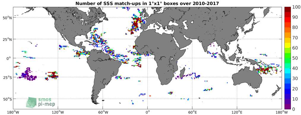
Figure 3: Number of SSS match-ups between Surface drifters SSS and the SMOS-L2-DPGS-v662 SSS product for the SMOS coastal zone ( \geq 800\text{km} ) 60N-60S Pi-MEP region over 1^\circ \times 1^\circ boxes and for the full satellite product period.
