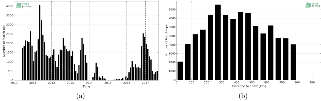
Figure 1: Number of match-ups between Surface drifters and SMOS-L2-DPGS-v662 SSS as a function of time (a) and as function of the distance to coast (b) over the SMOS coastal zone ( \pm 800\text{km} ) 60N-60S Pi-MEP region and for the full satellite product period.
