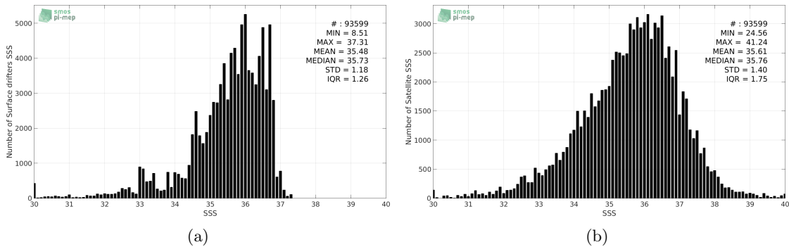
Figure 2: Histograms of SSS from Surface drifters (a) and SMOS-L2-DPGS-v662 (b) considering all match-up pairs per bins of 0.1 over the SMOS coastal zone ( \pm 800\text{km} ) 60N-60S Pi-MEP region and for the full satellite product period.
