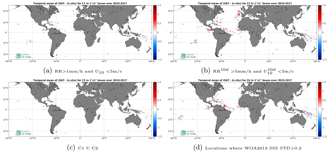
Figure 11: Temporal mean gridded over spatial boxes of size 1^\circ \times 1^\circ of \Delta SSS (SMOS-L2-DPGS-v662 - Surface drifters) for 4 different subdatasets corresponding to: RR > 1\text{mm/h} and U_{10} < 5\text{m/s} (a), RR^{10d} > 5\text{mm/h} and U_{10}^{10d} < 5\text{m/s} (b), C1 U C2 (c), Locations where WOA2013 SSS STD > 0.2 (d).
