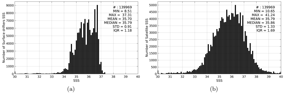
Figure 2: Histograms of SSS from Surface drifters (a) and SMOS-L2-DPGS-v662 (b) considering all match-up pairs per bins of 0.1 over the SMOS coastal zone ( \pm 800\text{km} ) 60N-60S Pi-MEP region and for the full satellite product period.
