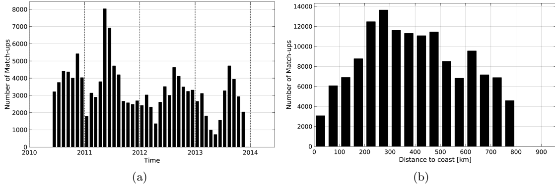
Figure 1: Number of match-ups between Surface drifters and SMOS-L2-DPGS-v662 SSS as a function of time (a) and as function of the distance to coast (b) over the SMOS coastal zone ( \pm 800\text{km} ) 60N-60S Pi-MEP region and for the full satellite product period.
