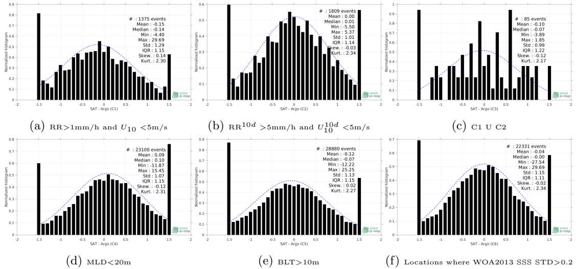
Figure 13: Normalized histogram of \Delta SSS (SMOS-L2-DPGS-v662 - Argo) for 6 different subdatasets corresponding to: RR > 1\text{mm/h} and U_{10} < 5\text{m/s} (a), RR^{10d} > 5\text{mm/h} and U_{10}^{10d} < 5\text{m/s} (b), C1 U C2 (c), MLD < 20\text{m} (d), BLT > 10\text{m} (e), Locations where WOA2013 SSS STD > 0.2 (f).
