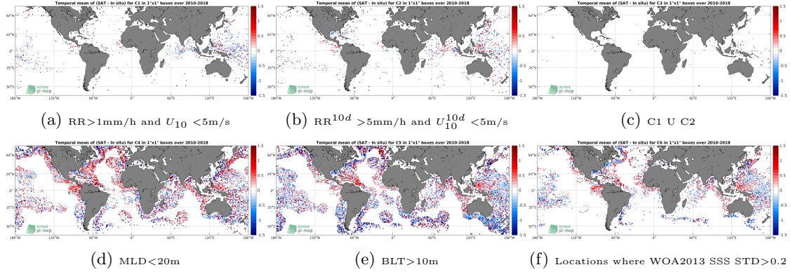
Figure 12: Temporal mean gridded over spatial boxes of size 1^\circ \times 1^\circ of \Delta SSS (SMOS-L2-DPGS-v662 - Argo) for 6 different subdatasets corresponding to: RR > 1\text{mm/h} and U_{10} < 5\text{m/s} (a), RR^{10d} > 5\text{mm/h} and U_{10}^{10d} < 5\text{m/s} (b), C1 U C2 (c), MLD < 20\text{m} (d), BLT > 10\text{m} (e), Locations where WOA2013 SSS STD > 0.2 (f).
