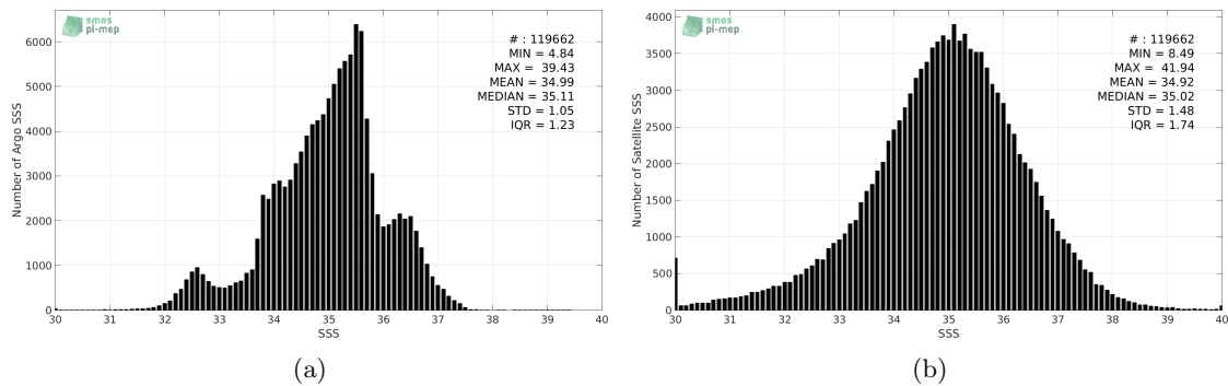
Figure 2: Histograms of SSS from Argo (a) and SMOS-L2-DPGS-v662 (b) considering all match-up pairs per bins of 0.1 over the SMOS coastal zone ( \geq 800 km) 60N-60S Pi-MEP region and for the full satellite product period.
