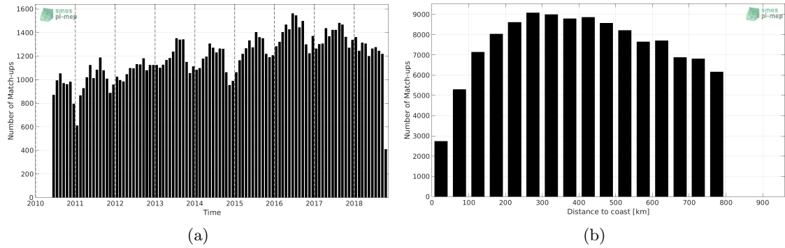
Figure 1: Number of match-ups between Argo and SMOS-L2-DPGS-v662 SSS as a function of time (a) and as function of the distance to coast (b) over the SMOS coastal zone ( \geq 800 km) 60N-60S Pi-MEP region and for the full satellite product period.
