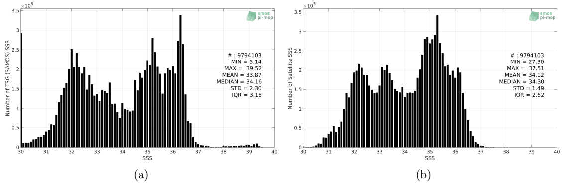
Figure 2: Histograms of SSS from TSG (SAMOS) (a) and SMAP SSS L4 OI v1 - 7 Days (IPRC) (b) considering all match-up pairs per bins of 0.1 over the SMOS coastal zone (<800km) 60N-60S Pi-MEP region and for the full satellite product period.
