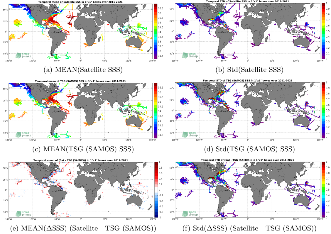
Figure 6: Temporal mean (left) and Std (right) of SSS from SMAP SSS L4 OI v1 - 7 Days (IPRC) (top), TSG (SAMOS) (middle), and of \Delta SSS (Satellite - TSG (SAMOS)). Only match-up pairs are used to generate these maps.
