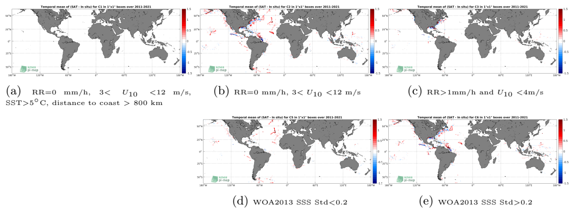
Figure 12: Temporal mean gridded over spatial boxes of size 1^\circ \times 1^\circ of \Delta SSS (SMAP SSS L4 OI v1 - 7 Days (IPRC) - TSG (SAMOS)) for 5 different subdatasets corresponding to:RR=0 mm/h, 3 < U_{10} < 12 m/s, SST >5^\circ\text{C} , distance to coast > 800 km (a), RR=0 mm/h, 3 < U_{10} < 12 m/s (b), RR >1 mm/h and U_{10} < 4 m/s (c), WOA2013 SSS Std <0.2 (d), WOA2013 SSS Std >0.2 (e).
