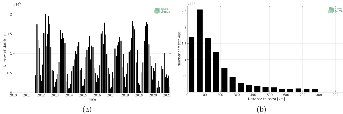
Figure 1: Number of match-ups between TSG (SAMOS) and SMAP SSS L4 OI v1 - 7 Days (IPRC) SSS as a function of time (a) and as function of the distance to coast (b) over the SMOS coastal zone (<800km) 60N-60S Pi-MEP region and for the full satellite product period.
