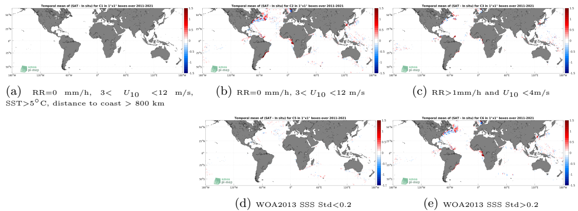
Figure 12: Temporal mean gridded over spatial boxes of size 1^\circ \times 1^\circ of \Delta SSS (SMAP SSS L4 OI v1 - 7 Days (IPRC) - TSG (LEGOS-DM)) for 5 different subdatasets corresponding to:RR=0 mm/h, 3 < U_{10} < 12 m/s, SST > 5^\circ\text{C} , distance to coast > 800 km (a), RR=0 mm/h, 3 < U_{10} < 12 m/s (b), RR > 1 mm/h and U_{10} < 4 m/s (c), WOA2013 SSS Std < 0.2 (d), WOA2013 SSS Std > 0.2 (e).
