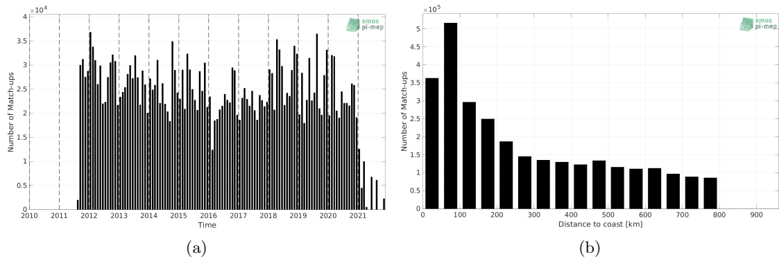
Figure 1: Number of match-ups between TSG (LEGOS-DM) and SMAP SSS L4 OI v1 - 7 Days (IPRC) SSS as a function of time (a) and as function of the distance to coast (b) over the SMOS coastal zone (<800km) 60N-60S Pi-MEP region and for the full satellite product period.
