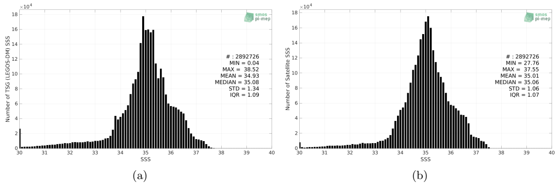
Figure 2: Histograms of SSS from TSG (LEGOS-DM) (a) and SMAP SSS L4 OI v1 - 7 Days (IPRC) (b) considering all match-up pairs per bins of 0.1 over the SMOS coastal zone (<800km) 60N-60S Pi-MEP region and for the full satellite product period.
