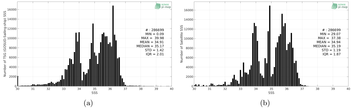
Figure 2: Histograms of SSS from TSG (GOSUD-Sailing-ship) (a) and SMAP SSS L4 OI v1 - 7 Days (IPRC) (b) considering all match-up pairs per bins of 0.1 over the SMOS coastal zone (<800km) 60N-60S Pi-MEP region and for the full satellite product period.
