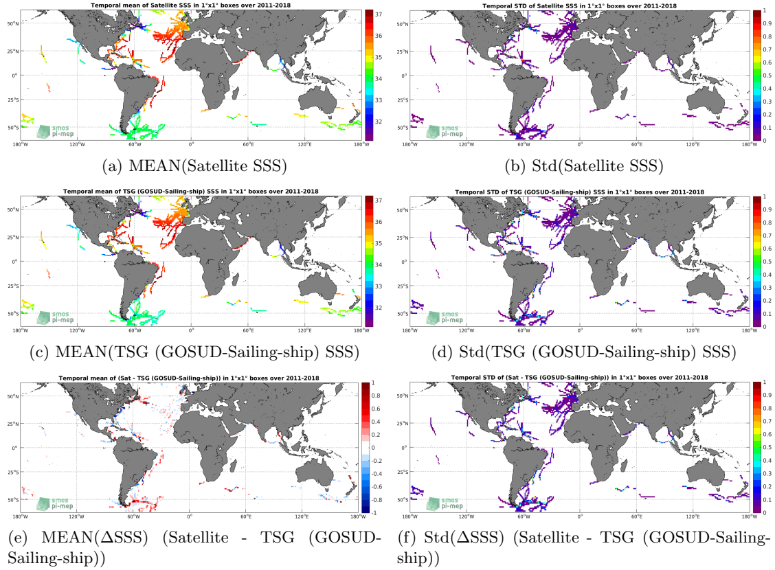
Figure 6: Temporal mean (left) and Std (right) of SSS from SMAP SSS L4 OI v1 - 7 Days (IPRC) (top), TSG (GOSUD-Sailing-ship) (middle), and of \Delta SSS (Satellite - TSG (GOSUD-Sailing-ship)). Only match-up pairs are used to generate these maps.
