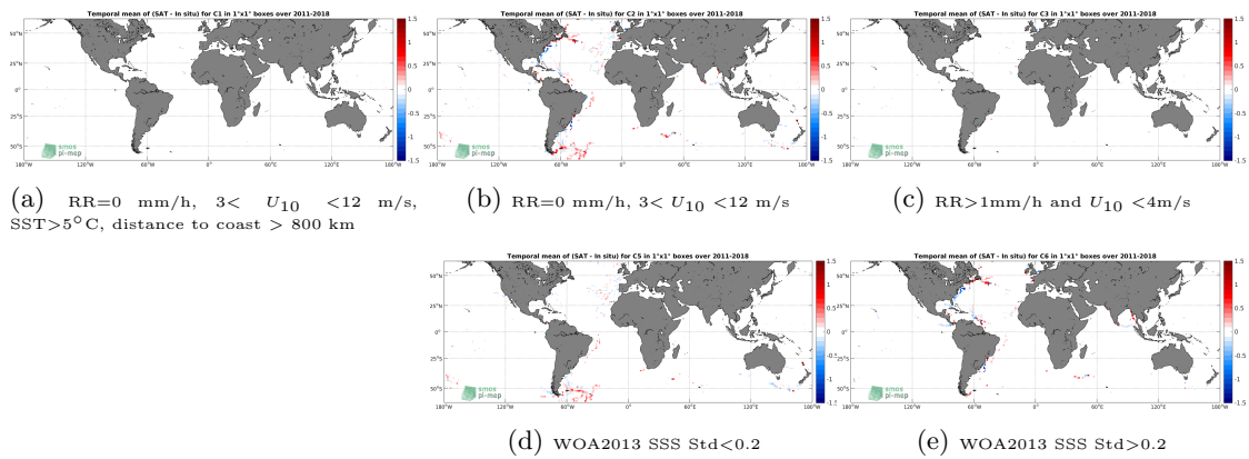
Figure 12: Temporal mean gridded over spatial boxes of size 1^\circ \times 1^\circ of \Delta SSS (SMAP SSS L4 OI v1 - 7 Days (IPRC) - TSG (GOSUD-Sailing-ship)) for 5 different subdatasets corresponding to:RR=0 mm/h, 3 < U_{10} < 12 m/s, SST>5°C, distance to coast > 800 km (a), RR=0 mm/h, 3 < U_{10} < 12 m/s (b), RR>1mm/h and U_{10} < 4 m/s (c), WOA2013 SSS Std<0.2 (d), WOA2013 SSS Std>0.2 (e).
