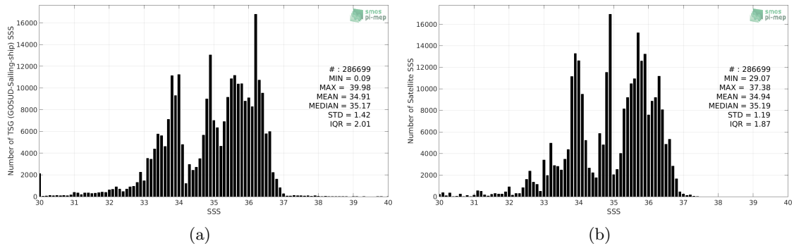
Figure 2: Histograms of SSS from TSG (GOSUD-Sailing-ship) (a) and SMAP SSS L4 OI v1 - 7day (IPRC) (b) considering all match-up pairs per bins of 0.1 over the SMOS coastal zone (<800km) 60N-60S Pi-MEP region and for the full satellite product period.
