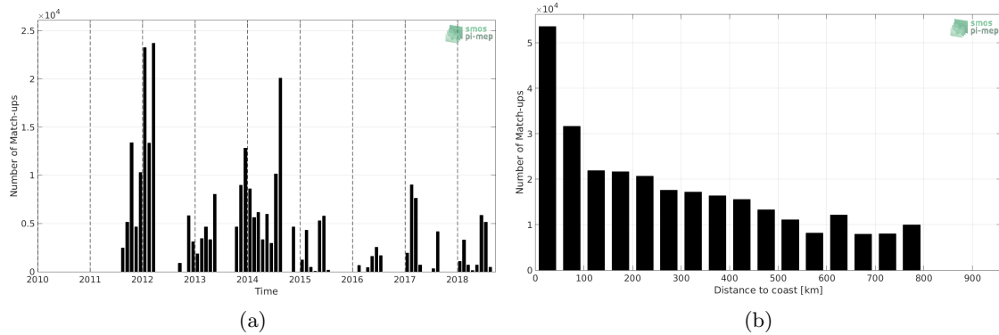
Figure 1: Number of match-ups between TSG (GOSUD-Sailing-ship) and SMAP SSS L4 OI v1 - 7day (IPRC) SSS as a function of time (a) and as function of the distance to coast (b) over the SMOS coastal zone (<800km) 60N-60S Pi-MEP region and for the full satellite product period.
