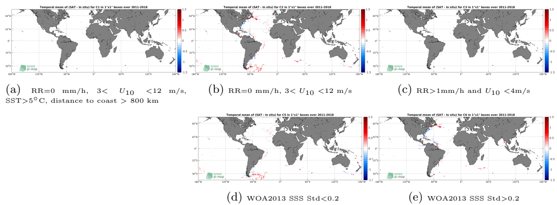
Figure 12: Temporal mean gridded over spatial boxes of size 1^\circ \times 1^\circ of \Delta SSS (SMAP SSS L4 OI v1 - 7day (IPRC) - TSG (GOSUD-Sailing-ship)) for 5 different subdatasets corresponding to:RR=0 mm/h, 3 < U_{10} < 12 m/s, SST>5°C, distance to coast > 800 km (a), RR=0 mm/h, 3 < U_{10} < 12 m/s (b), RR>1mm/h and U_{10} < 4 m/s (c), WOA2013 SSS Std<0.2 (d), WOA2013 SSS Std>0.2 (e).
