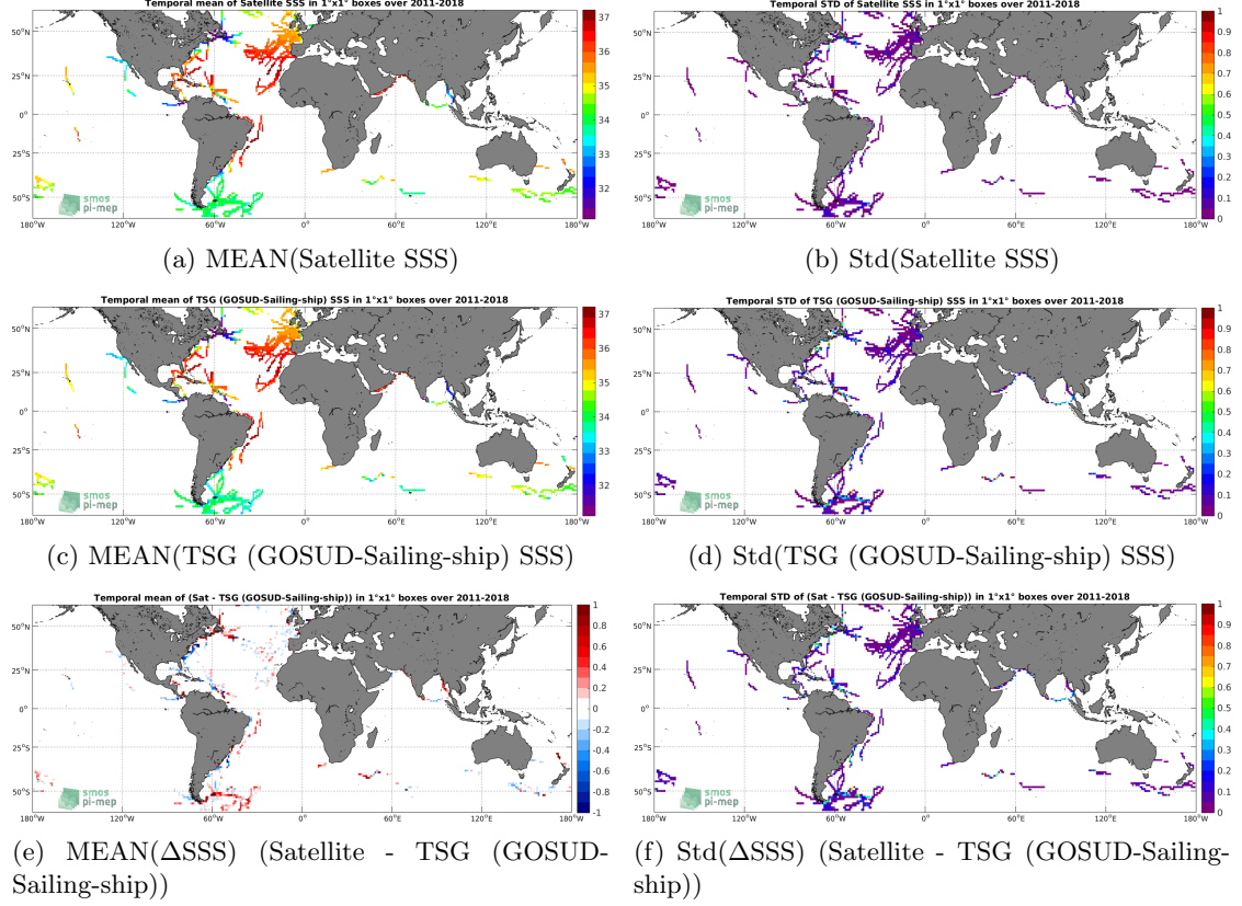
Figure 6: Temporal mean (left) and Std (right) of SSS from SMAP SSS L4 OI v1 - 7day (IPRC) (top), TSG (GOSUD-Sailing-ship) (middle), and of \Delta SSS (Satellite - TSG (GOSUD-Sailing-ship)). Only match-up pairs are used to generate these maps.
