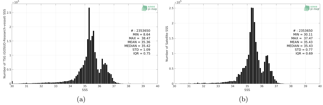
Figure 2: Histograms of SSS from TSG (GOSUD-Research-vessel) (a) and SMAP SSS L4 OI v1 - 7 Days (IPRC) (b) considering all match-up pairs per bins of 0.1 over the SMOS coastal zone (<800km) 60N-60S Pi-MEP region and for the full satellite product period.
