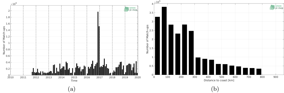
Figure 1: Number of match-ups between TSG (GOSUD-Research-vessel) and SMAP SSS L4 OI v1 - 7 Days (IPRC) SSS as a function of time (a) and as function of the distance to coast (b) over the SMOS coastal zone (<800km) 60N-60S Pi-MEP region and for the full satellite product period.
