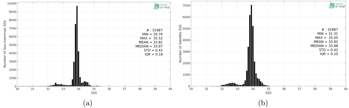
Figure 2: Histograms of SSS from Marine mammals (a) and SMAP SSS L4 OI v1 - 7 Days (IPRC) (b) considering all match-up pairs per bins of 0.1 over the SMOS coastal zone (<800km) 60N-60S Pi-MEP region and for the full satellite product period.
