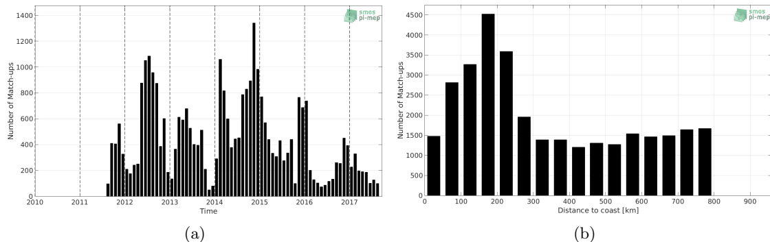
Figure 1: Number of match-ups between Marine mammals and SMAP SSS L4 OI v1 - 7 Days (IPRC) SSS as a function of time (a) and as function of the distance to coast (b) over the SMOS coastal zone (<800km) 60N-60S Pi-MEP region and for the full satellite product period.
