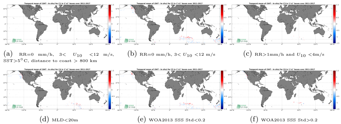
Figure 12: Temporal mean gridded over spatial boxes of size 1^\circ \times 1^\circ of \Delta SSS (SMAP SSS L4 OI v1 - 7 Days (IPRC) - Marine mammals) for 6 different subdatasets corresponding to:RR=0 mm/h, 3 < U_{10} < 12 m/s, SST > 5°C, distance to coast > 800 km (a), RR=0 mm/h, 3 < U_{10} < 12 m/s (b), RR > 1mm/h and U_{10} < 4 m/s (c),MLD < 20m (d),WOA2013 SSS Std < 0.2 (e),WOA2013 SSS Std > 0.2 (f).
