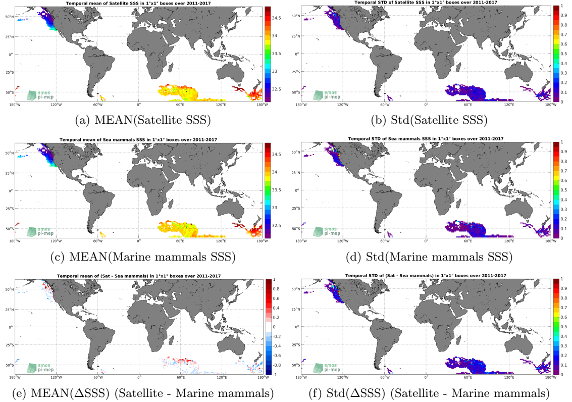
Figure 6: Temporal mean (left) and Std (right) of SSS from SMAP SSS L4 OI v1 - 7 Days (IPRC) (top), Marine mammals (middle), and of \Delta SSS (Satellite - Marine mammals). Only match-up pairs are used to generate these maps.
