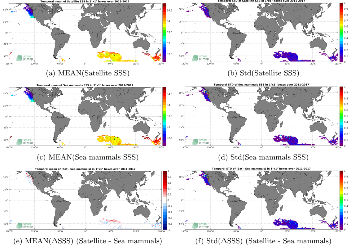
Figure 6: Temporal mean (left) and Std (right) of SSS from SMAP SSS L4 OI v1 - 7day (IPRC) (top), Sea mammals (middle), and of \Delta SSS (Satellite - Sea mammals). Only match-up pairs are used to generate these maps.
