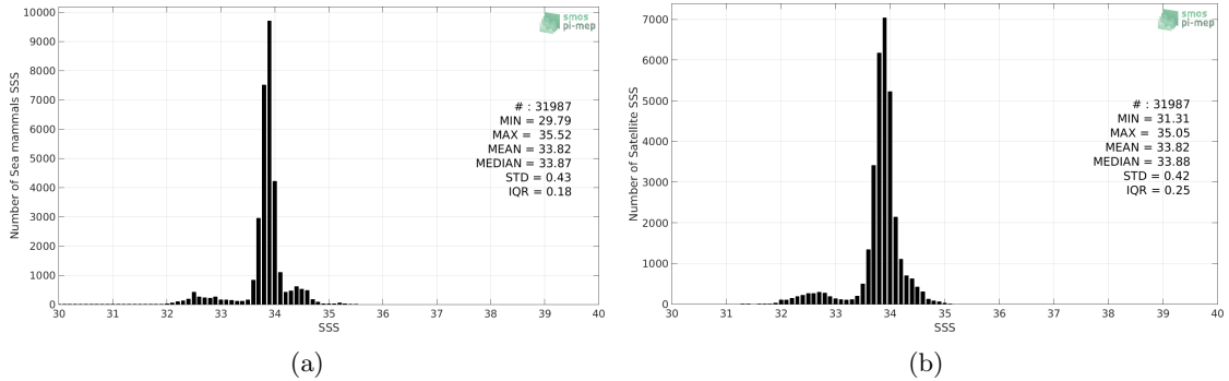
Figure 2: Histograms of SSS from Sea mammals (a) and SMAP SSS L4 OI v1 - 7day (IPRC) (b) considering all match-up pairs per bins of 0.1 over the SMOS coastal zone (<800km) 60N-60S Pi-MEP region and for the full satellite product period.
