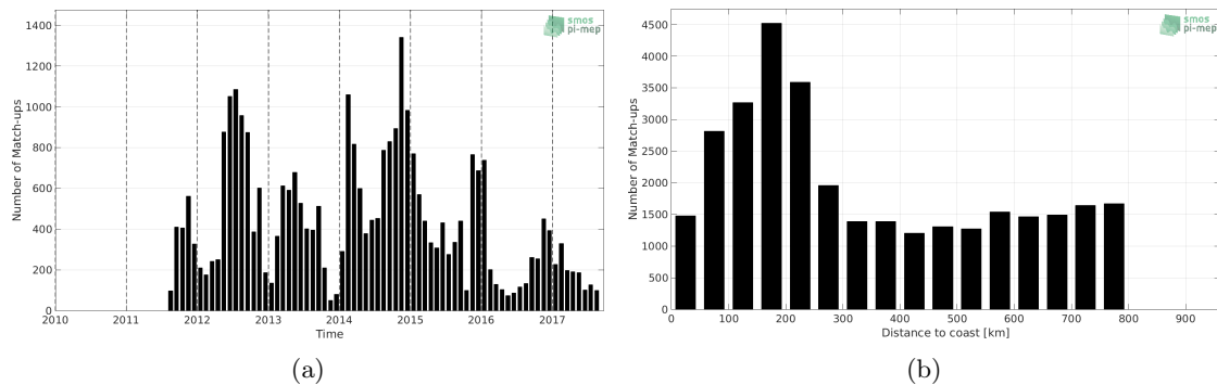
Figure 1: Number of match-ups between Sea mammals and SMAP SSS L4 OI v1 - 7day (IPRC) SSS as a function of time (a) and as function of the distance to coast (b) over the SMOS coastal zone (<800km) 60N-60S Pi-MEP region and for the full satellite product period.
