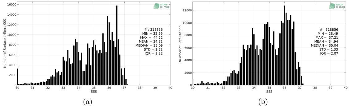
Figure 2: Histograms of SSS from Surface drifters (a) and SMAP SSS L4 OI v1 - 7 Days (IPRC) (b) considering all match-up pairs per bins of 0.1 over the SMOS coastal zone (<800km) 60N-60S Pi-MEP region and for the full satellite product period.
