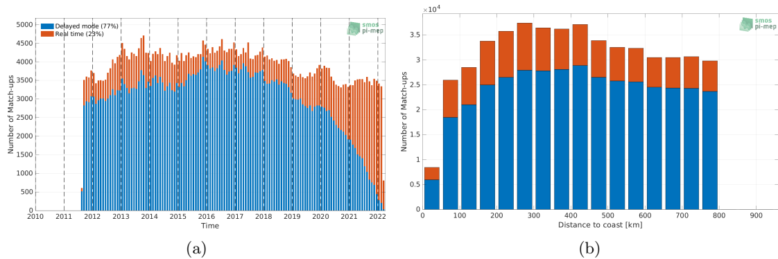
Figure 1: Number of match-ups between Argo and SMAP SSS L4 OI v1 - 7 Days (IPRC) SSS as a function of time (a) and as function of the distance to coast (b) over the SMOS coastal zone (<800km) 60N-60S Pi-MEP region and for the full satellite product period.
