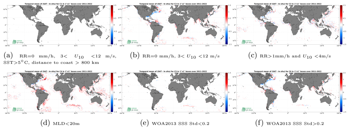
Figure 12: Temporal mean gridded over spatial boxes of size 1^\circ \times 1^\circ of \Delta SSS (SMAP SSS L4 OI v1 - 7 Days (IPRC) - Argo) for 6 different subdatasets corresponding to:RR=0 mm/h, 3 < U_{10} < 12 m/s, SST > 5^\circ C, distance to coast > 800 km (a), RR=0 mm/h, 3 < U_{10} < 12 m/s (b), RR > 1 mm/h and U_{10} < 4 m/s (c),MLD < 20 m (d),WOA2013 SSS Std < 0.2 (e),WOA2013 SSS Std > 0.2 (f).
