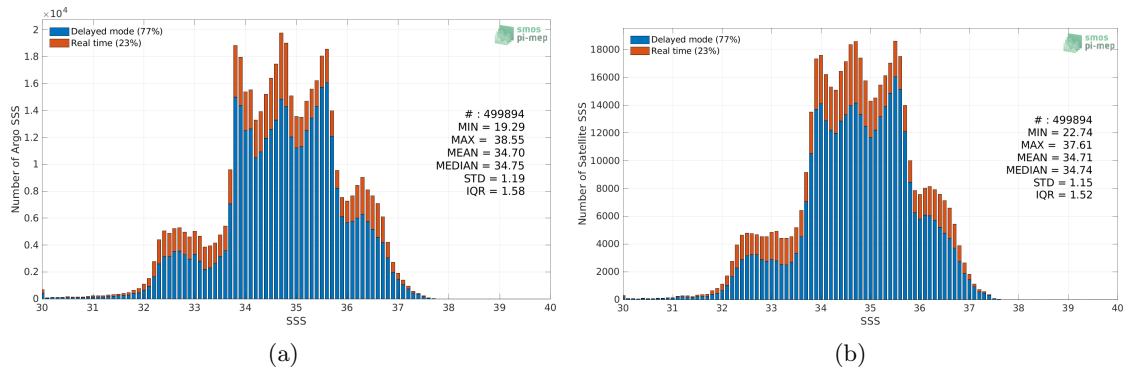
Figure 2: Histograms of SSS from Argo (a) and SMAP SSS L4 OI v1 - 7 Days (IPRC) (b) considering all match-up pairs per bins of 0.1 over the SMOS coastal zone (<800km) 60N-60S Pi-MEP region and for the full satellite product period.
