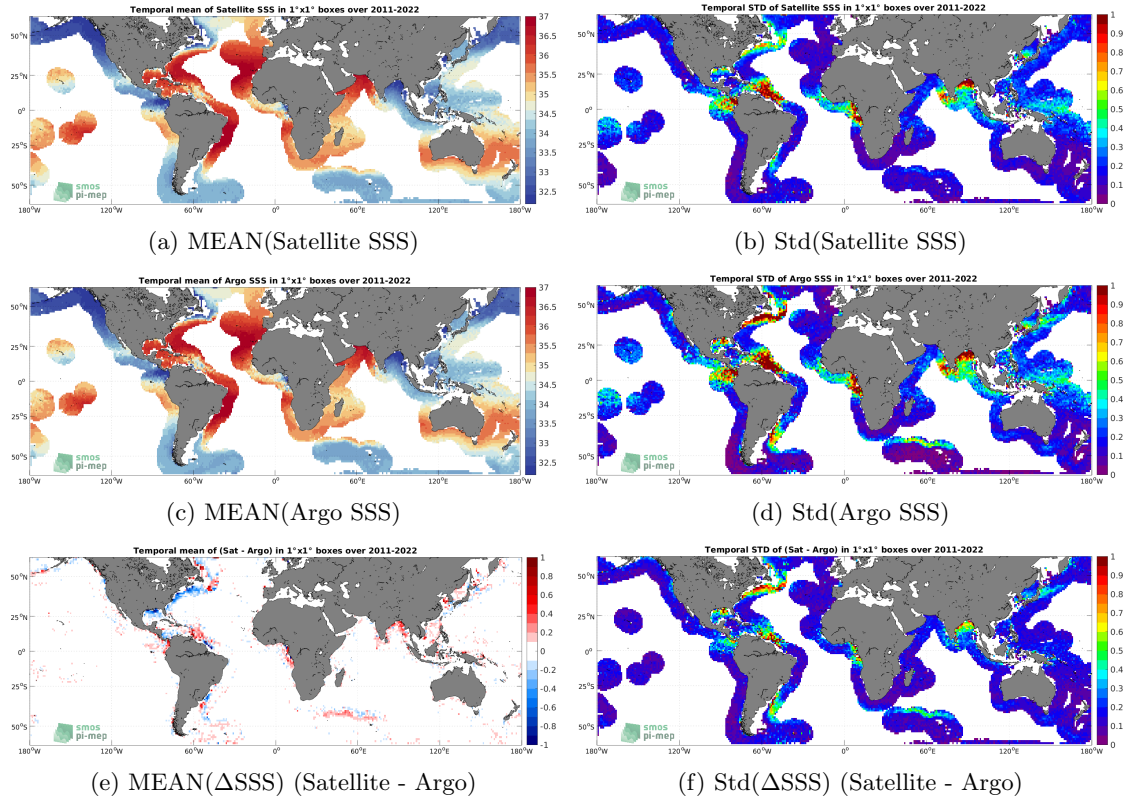
Figure 6: Temporal mean (left) and Std (right) of SSS from SMAP SSS L4 OI v1 - 7 Days (IPRC) (top), Argo (middle), and of \Delta SSS (Satellite - Argo). Only match-up pairs are used to generate these maps.
