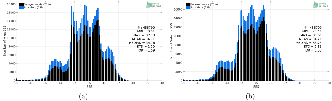
Figure 2: Histograms of SSS from Argo (a) and SMAP SSS L4 OI v1 - 7 Days (IPRC) (b) considering all match-up pairs per bins of 0.1 over the SMOS coastal zone (<800km) 60N-60S Pi-MEP region and for the full satellite product period.
