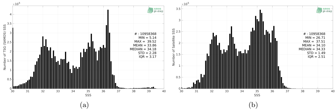
Figure 2: Histograms of SSS from TSG (SAMOS) (a) and SMAP SSS L4 OI v1 - Monthly (IPRC) (b) considering all match-up pairs per bins of 0.1 over the SMOS coastal zone (<800km) 60N-60S Pi-MEP region and for the full satellite product period.
