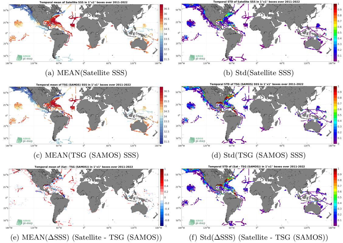
Figure 6: Temporal mean (left) and Std (right) of SSS from SMAP SSS L4 OI v1 - Monthly (IPRC) (top), TSG (SAMOS) (middle), and of \Delta SSS (Satellite - TSG (SAMOS)). Only match-up pairs are used to generate these maps.
