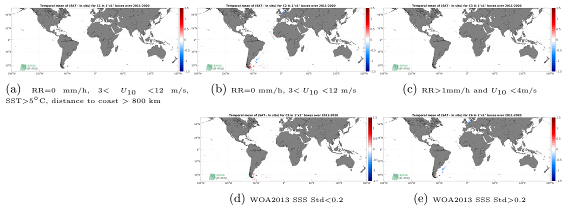
Figure 12: Temporal mean gridded over spatial boxes of size 1^\circ \times 1^\circ of \Delta SSS (SMAP SSS L4 OI v1 - Monthly (IPRC) - TSG (Polarstern)) for 5 different subdatasets corresponding to:RR=0 mm/h, 3 < U_{10} < 12 m/s, SST >5^\circ\text{C} , distance to coast > 800 km (a), RR=0 mm/h, 3 < U_{10} < 12 m/s (b), RR >1 mm/h and U_{10} < 4 m/s (c), WOA2013 SSS Std <0.2 (d), WOA2013 SSS Std >0.2 (e).
