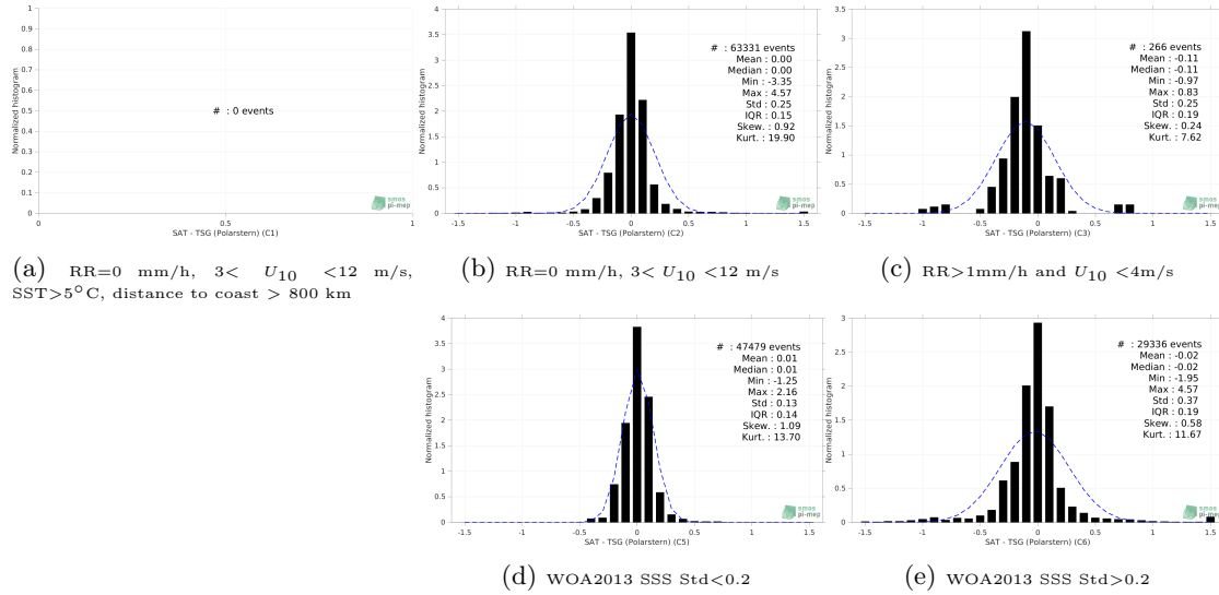
Figure 13: Normalized histogram of \Delta SSS (SMAP SSS L4 OI v1 - Monthly (IPRC) - TSG (Polarstern)) for 5 different subdatasets corresponding to: RR=0 mm/h, 3 < U_{10} < 12 m/s, SST > 5°C, distance to coast > 800 km (a), RR=0 mm/h, 3 < U_{10} < 12 m/s (b), RR > 1mm/h and U_{10} < 4 m/s (c), WOA2013 SSS Std < 0.2 (d), WOA2013 SSS Std > 0.2 (e).
