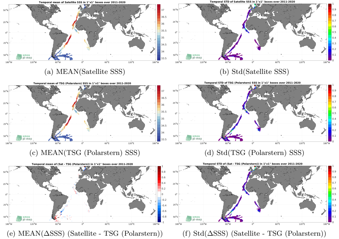
Figure 6: Temporal mean (left) and Std (right) of SSS from SMAP SSS L4 OI v1 - Monthly (IPRC) (top), TSG (Polarstern) (middle), and of \Delta SSS (Satellite - TSG (Polarstern)). Only match-up pairs are used to generate these maps.
