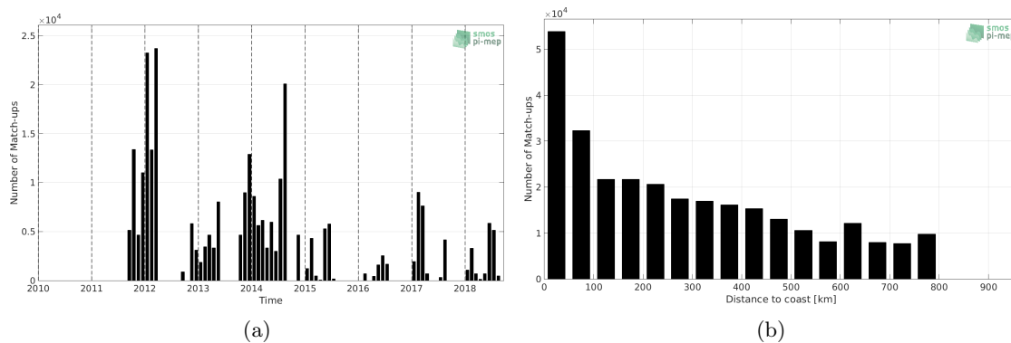
Figure 1: Number of match-ups between TSG (GOSUD-Sailing-ship) and SMAP SSS L4 OI v1 - Monthly (IPRC) SSS as a function of time (a) and as function of the distance to coast (b) over the SMOS coastal zone (<800km) 60N-60S Pi-MEP region and for the full satellite product period.
