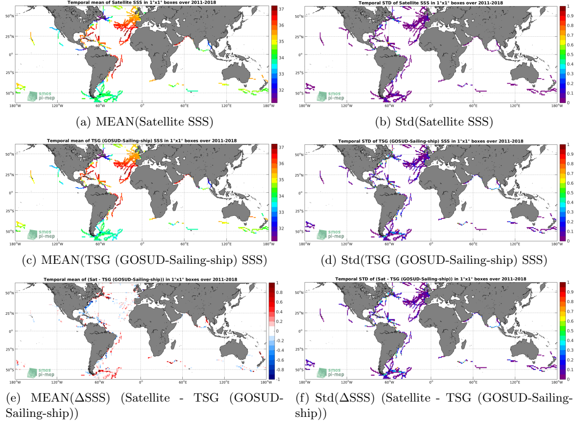
Figure 6: Temporal mean (left) and Std (right) of SSS from SMAP SSS L4 OI v1 - Monthly (IPRC) (top), TSG (GOSUD-Sailing-ship) (middle), and of \Delta SSS (Satellite - TSG (GOSUD-Sailing-ship)). Only match-up pairs are used to generate these maps.
