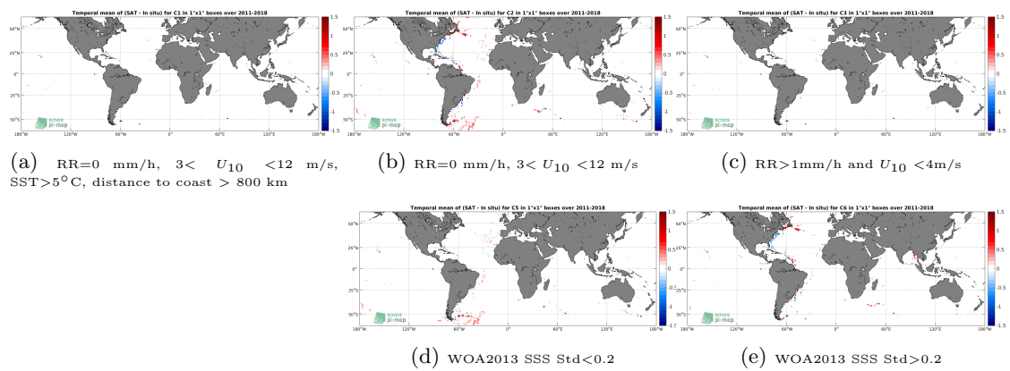
Figure 12: Temporal mean gridded over spatial boxes of size 1^\circ \times 1^\circ of \Delta\text{SSS} (SMAP SSS L4 OI v1 - Monthly (IPRC) - TSG (GOSUD-Sailing-ship)) for 5 different subdatasets corresponding to:RR=0 mm/h, 3 < U_{10} < 12 m/s, SST>5°C, distance to coast > 800 km (a), RR=0 mm/h, 3 < U_{10} < 12 m/s (b), RR>1mm/h and U_{10} < 4 m/s (c), WOA2013 SSS Std<0.2 (d), WOA2013 SSS Std>0.2 (e).
