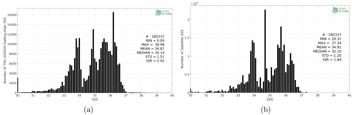
Figure 2: Histograms of SSS from TSG (GOSUD-Sailing-ship) (a) and SMAP SSS L4 OI v1 - Monthly (IPRC) (b) considering all match-up pairs per bins of 0.1 over the SMOS coastal zone (<800km) 60N-60S Pi-MEP region and for the full satellite product period.
