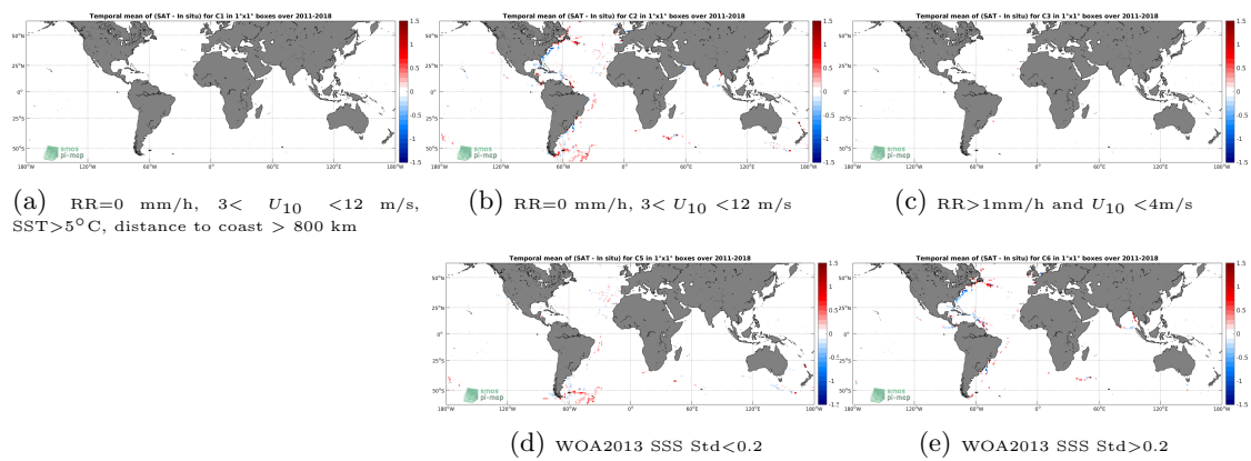
Figure 12: Temporal mean gridded over spatial boxes of size 1^\circ \times 1^\circ of \Delta SSS (SMAP SSS L4 OI v1 - Monthly (IPRC) - TSG (GOSUD-Sailing-ship)) for 5 different subdatasets corresponding to: RR=0 mm/h, 3 < U_{10} < 12 m/s, SST > 5°C, distance to coast > 800 km (a), RR=0 mm/h, 3 < U_{10} < 12 m/s (b), RR > 1mm/h and U_{10} < 4 m/s (c), WOA2013 SSS Std < 0.2 (d), WOA2013 SSS Std > 0.2 (e).
