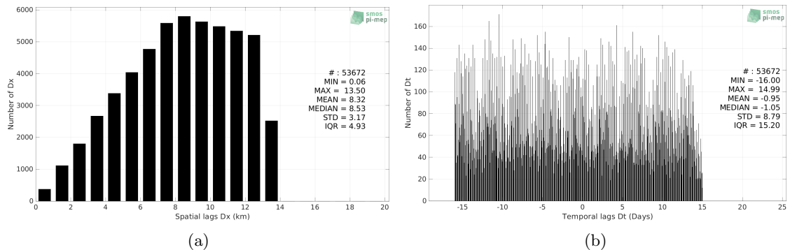
Figure 5: Histograms of the spatial (a) and temporal (b) lags between the location/time of the Marine mammals pixel measurement and the date of the corresponding SMAP SSS L4 OI v1 - Monthly (IPRC) SSS pixel.
