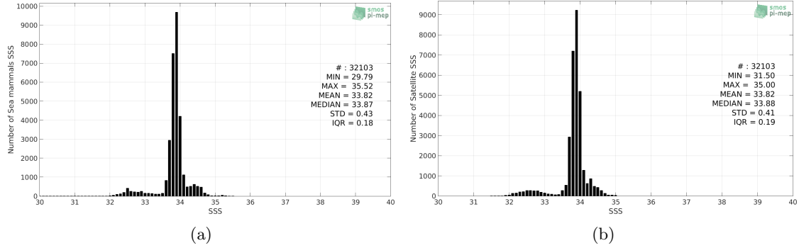
Figure 2: Histograms of SSS from Marine mammals (a) and SMAP SSS L4 OI v1 - Monthly (IPRC) (b) considering all match-up pairs per bins of 0.1 over the SMOS coastal zone (<800km) 60N-60S Pi-MEP region and for the full satellite product period.
