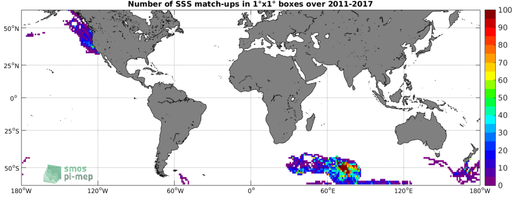
Figure 4: Number of SSS match-ups between Marine mammals SSS and the SMAP SSS L4 OI v1 - Monthly (IPRC) SSS product for the SMOS coastal zone (<800km) 60N-60S Pi-MEP region over 1^\circ \times 1^\circ boxes and for the full satellite product period.
