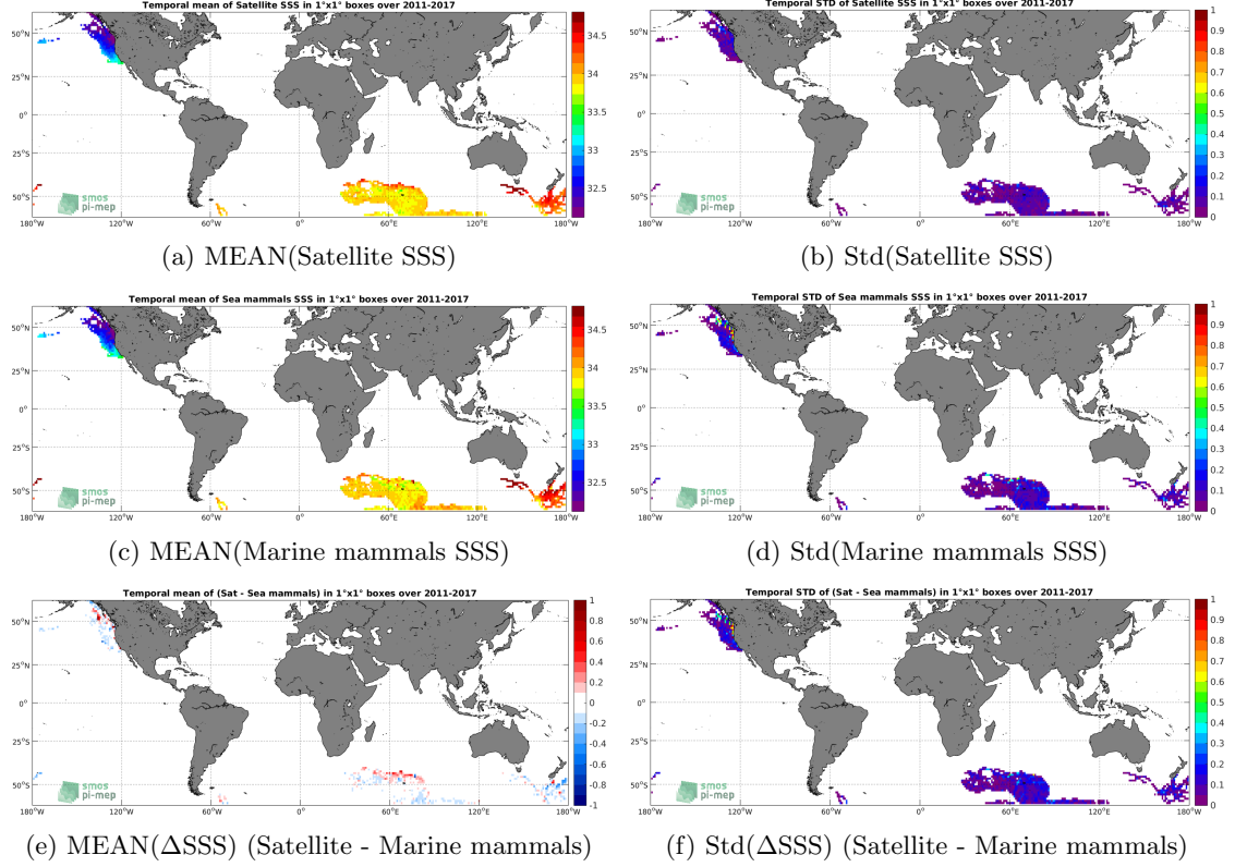
Figure 6: Temporal mean (left) and Std (right) of SSS from SMAP SSS L4 OI v1 - Monthly (IPRC) (top), Marine mammals (middle), and of \Delta SSS (Satellite - Marine mammals). Only match-up pairs are used to generate these maps.
