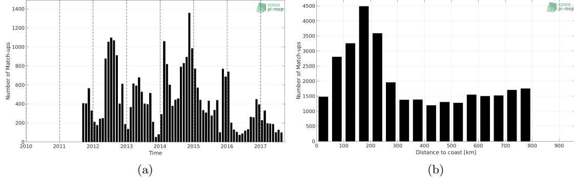
Figure 1: Number of match-ups between Marine mammals and SMAP SSS L4 OI v1 - Monthly (IPRC) SSS as a function of time (a) and as function of the distance to coast (b) over the SMOS coastal zone (<800km) 60N-60S Pi-MEP region and for the full satellite product period.
