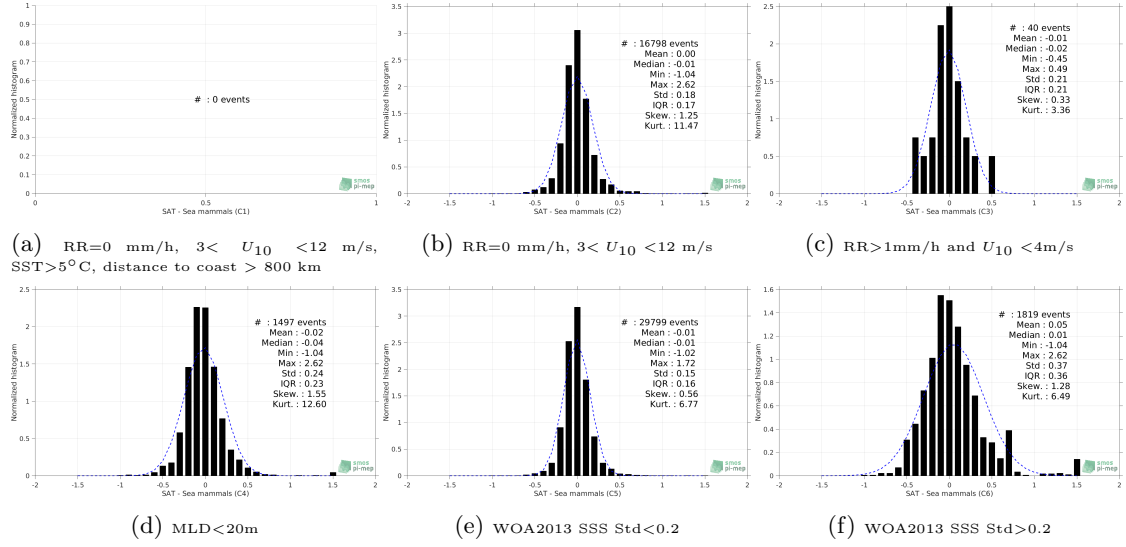
Figure 13: Normalized histogram of \Delta SSS (SMAP SSS L4 OI v1 - Monthly (IPRC) - Marine mammals) for 6 different subdatasets corresponding to: RR=0 mm/h, 3 < U_{10} < 12 m/s, SST>5°C, distance to coast > 800 km (a), RR=0 mm/h, 3 < U_{10} < 12 m/s (b), RR>1mm/h and U_{10} < 4 m/s (c), MLD<20m (d), WOA2013 SSS Std<0.2 (e), WOA2013 SSS Std>0.2 (f).
