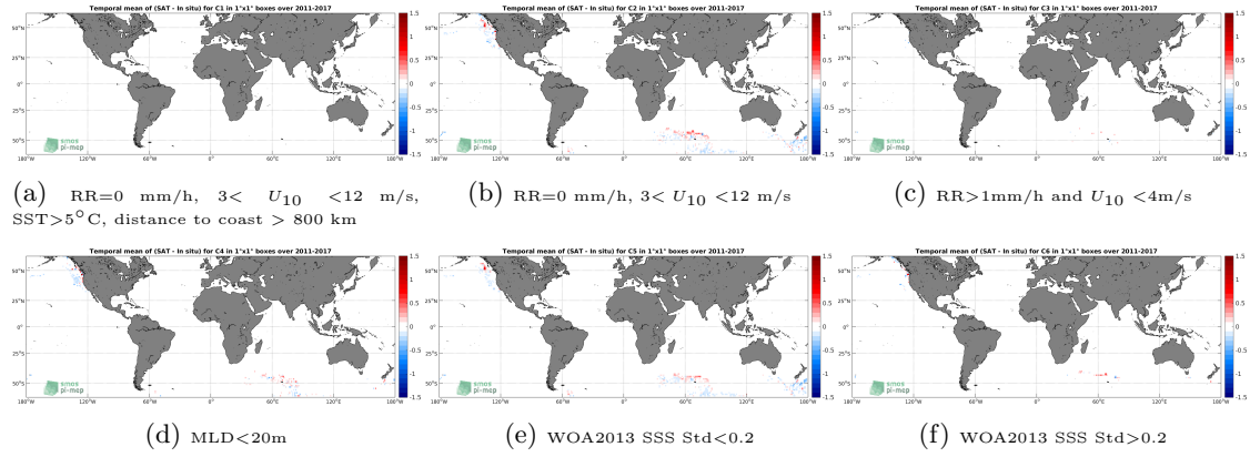
Figure 12: Temporal mean gridded over spatial boxes of size 1^\circ \times 1^\circ of \Delta SSS (SMAP SSS L4 OI v1 - Monthly (IPRC) - Marine mammals) for 6 different subdatasets corresponding to: RR=0 mm/h, 3 < U_{10} < 12 m/s, SST > 5^\circ C , distance to coast > 800 km (a), RR=0 mm/h, 3 < U_{10} < 12 m/s (b), RR > 1 mm/h and U_{10} < 4 m/s (c), MLD < 20 m (d), WOA2013 SSS Std < 0.2 (e), WOA2013 SSS Std > 0.2 (f).
