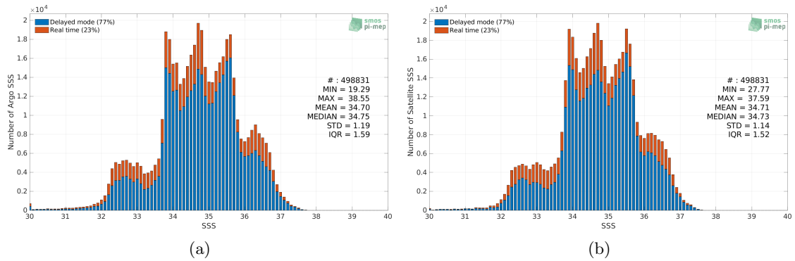
Figure 2: Histograms of SSS from Argo (a) and SMAP SSS L4 OI v1 - Monthly (IPRC) (b) considering all match-up pairs per bins of 0.1 over the SMOS coastal zone (<800km) 60N-60S Pi-MEP region and for the full satellite product period.
