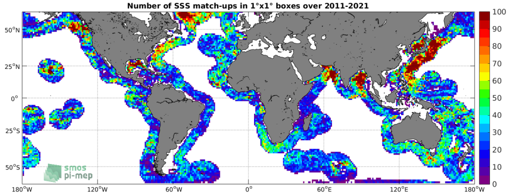
Figure 4: Number of SSS match-ups between Argo SSS and the SMAP SSS L4 OI v1 - Monthly (IPRC) SSS product for the SMOS coastal zone (<800km) 60N-60S Pi-MEP region over 1^{\circ} \times 1^{\circ} boxes and for the full satellite product period.
