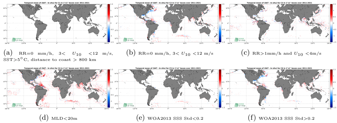
Figure 12: Temporal mean gridded over spatial boxes of size 1^\circ \times 1^\circ of \Delta SSS (SMAP SSS L4 OI v1 - Monthly (IPRC) - Argo) for 6 different subdatasets corresponding to: RR=0 mm/h, 3 < U_{10} < 12 m/s, SST > 5°C, distance to coast > 800 km (a), RR=0 mm/h, 3 < U_{10} < 12 m/s (b), RR > 1mm/h and U_{10} < 4 m/s (c), MLD < 20m (d), WOA2013 SSS Std < 0.2 (e), WOA2013 SSS Std > 0.2 (f).
