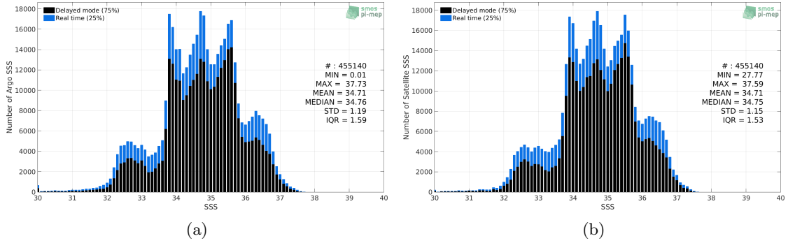
Figure 2: Histograms of SSS from Argo (a) and SMAP SSS L4 OI v1 - Monthly (IPRC) (b) considering all match-up pairs per bins of 0.1 over the SMOS coastal zone (<800km) 60N-60S Pi-MEP region and for the full satellite product period.
