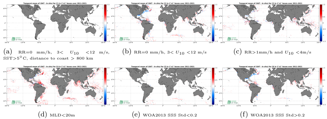
Figure 12: Temporal mean gridded over spatial boxes of size 1°x1° of \Delta SSS (SMAP SSS L4 OI v1 - Monthly (IPRC) - Argo) for 6 different subdatasets corresponding to:RR=0 mm/h, 3 < U_{10} < 12 m/s, SST > 5°C, distance to coast > 800 km (a), RR=0 mm/h, 3 < U_{10} < 12 m/s (b), RR > 1mm/h and U_{10} < 4 m/s (c),MLD < 20m (d),WOA2013 SSS Std < 0.2 (e),WOA2013 SSS Std > 0.2 (f).
