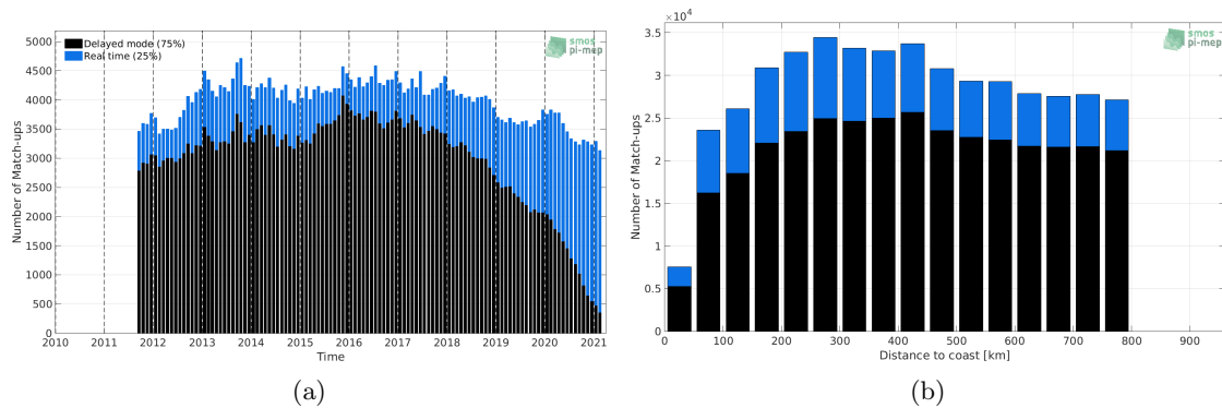
Figure 1: Number of match-ups between Argo and SMAP SSS L4 OI v1 - Monthly (IPRC) SSS as a function of time (a) and as function of the distance to coast (b) over the SMOS coastal zone (<800km) 60N-60S Pi-MEP region and for the full satellite product period.
