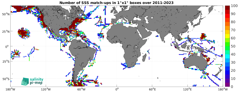
Figure 5: Number of SSS match-ups between TSG (SAMOS) SSS and the SMAP SSS L4 OI v3 - Monthly (ESR) SSS product for the SMOS coastal zone (<800km) 60N-60S Pi-MEP region over 1^\circ \times 1^\circ boxes and for the full satellite product period.
