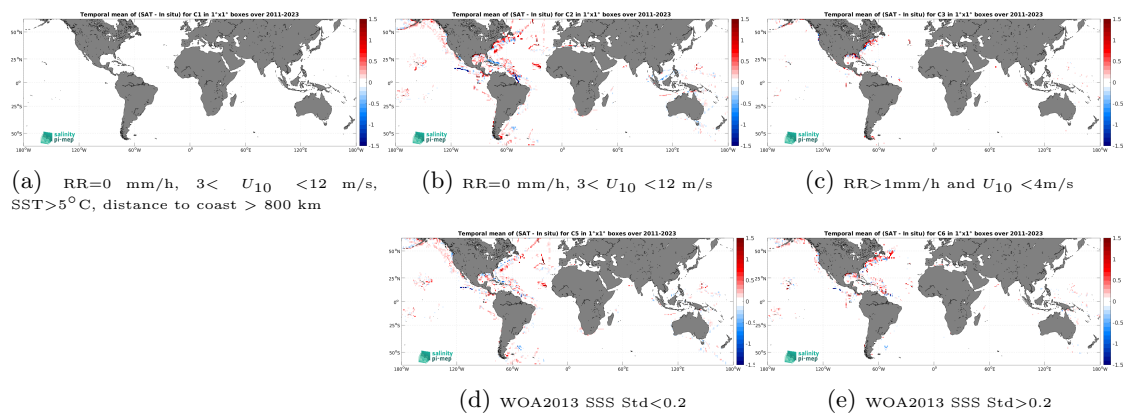
Figure 14: Temporal mean gridded over spatial boxes of size 1^\circ \times 1^\circ of \Delta SSS (SMAP SSS L4 OI v3 - Monthly (ESR) - TSG (SAMOS)) for 5 different subdatasets corresponding to:RR=0 mm/h, 3 < U_{10} < 12 m/s, SST >5^\circ\text{C} , distance to coast > 800 km (a), RR=0 mm/h, 3 < U_{10} < 12 m/s (b), RR >1 mm/h and U_{10} < 4 m/s (c), WOA2013 SSS Std <0.2 (d), WOA2013 SSS Std >0.2 (e).
