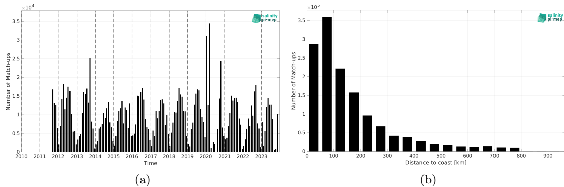
Figure 2: Number of match-ups between TSG (SAMOS) and SMAP SSS L4 OI v3 - Monthly (ESR) SSS as a function of time (a) and as function of the distance to coast (b) over the SMOS coastal zone ( < 800\text{km} ) 60N-60S Pi-MEP region and for the full satellite product period.
