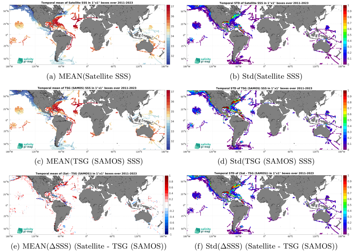
Figure 7: Temporal mean (left) and Std (right) of SSS from SMAP SSS L4 OI v3 - Monthly (ESR) (top), TSG (SAMOS) (middle), and of \Delta SSS (Satellite - TSG (SAMOS)). Only match-up pairs are used to generate these maps.
