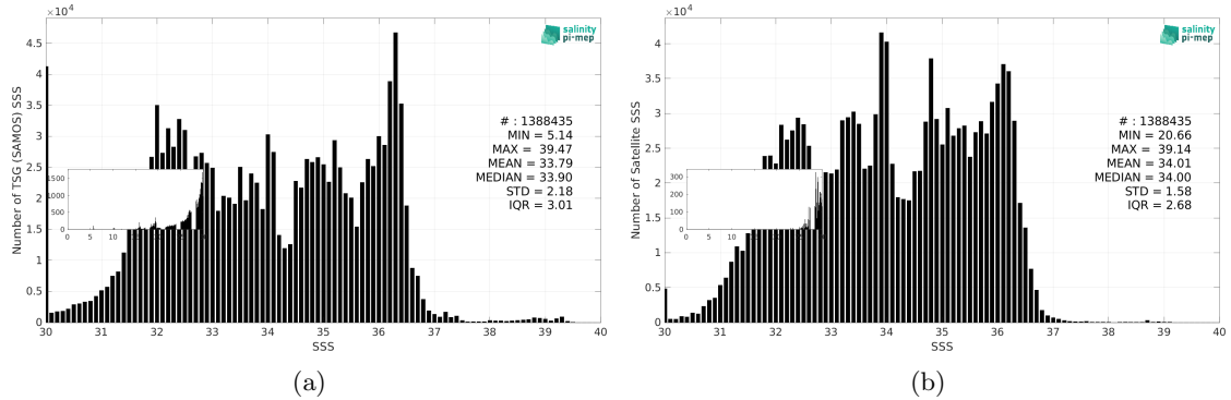
Figure 3: Histograms of SSS from TSG (SAMOS) (a) and SMAP SSS L4 OI v3 - Monthly (ESR) (b) considering all match-up pairs per bins of 0.1 over the SMOS coastal zone (<800km) 60N-60S Pi-MEP region and for the full satellite product period.
