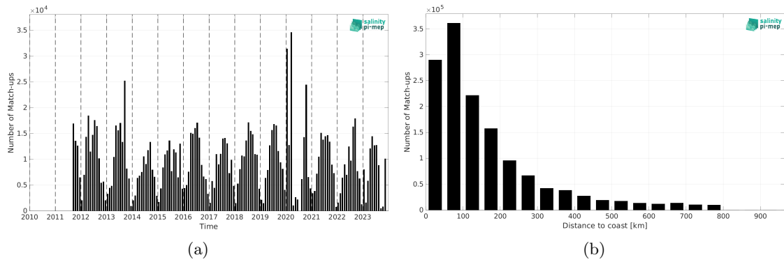
Figure 2: Number of match-ups between TSG (SAMOS) and SMAP SSS L4 OI v3 - Monthly (ESR) SSS as a function of time (a) and as function of the distance to coast (b) over the SMOS coastal zone (<800km) 60N-60S Pi-MEP region and for the full satellite product period.
