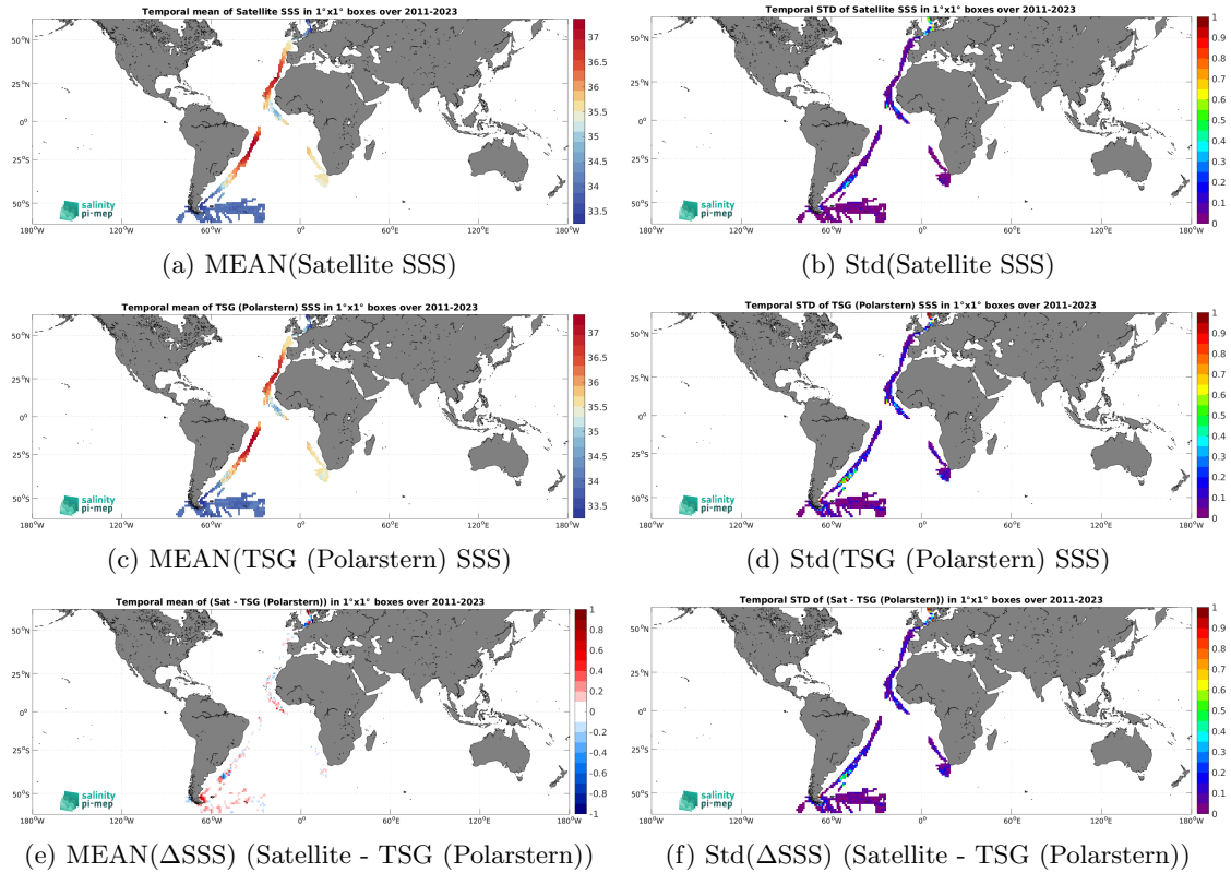
Figure 7: Temporal mean (left) and Std (right) of SSS from SMAP SSS L4 OI v3 - Monthly (ESR) (top), TSG (Polarstern) (middle), and of \Delta SSS (Satellite - TSG (Polarstern)). Only match-up pairs are used to generate these maps.
