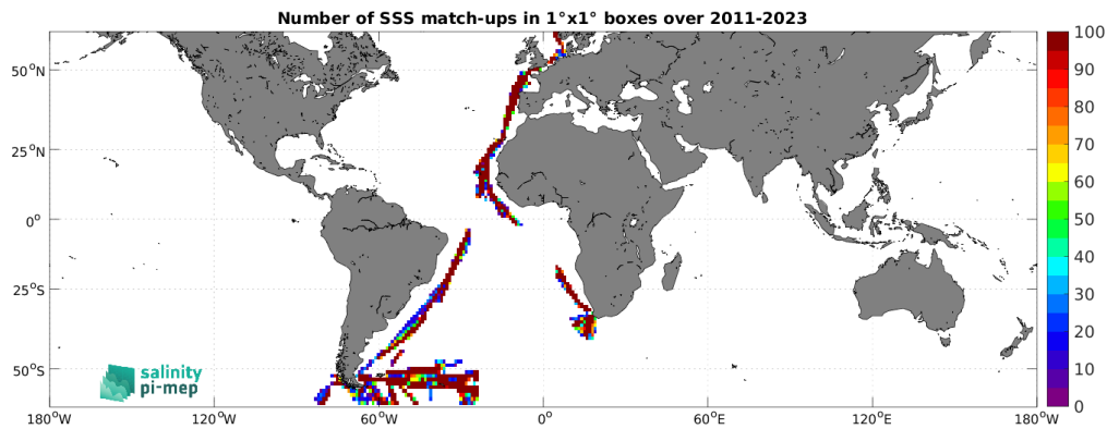
Figure 5: Number of SSS match-ups between TSG (Polarstern) SSS and the SMAP SSS L4 OI v3 - Monthly (ESR) SSS product for the SMOS coastal zone (<800km) 60N-60S Pi-MEP region over 1^\circ \times 1^\circ boxes and for the full satellite product period.
