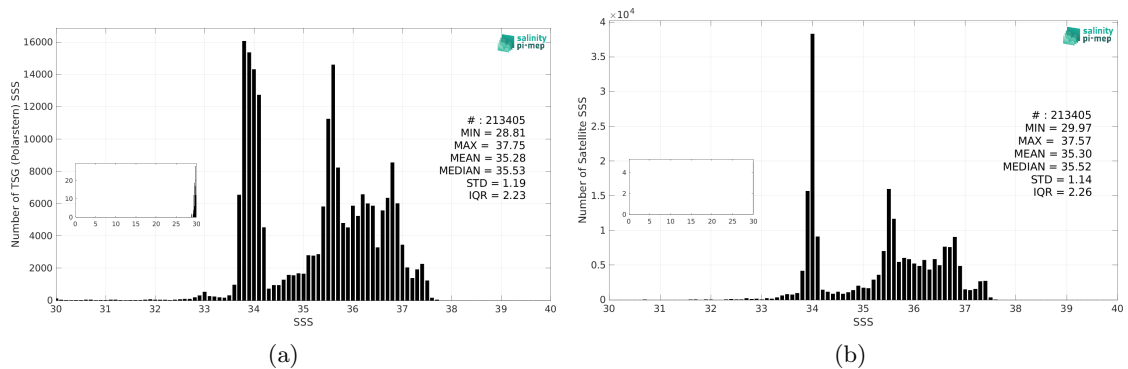
Figure 3: Histograms of SSS from TSG (Polarstern) (a) and SMAP SSS L4 OI v3 - Monthly (ESR) (b) considering all match-up pairs per bins of 0.1 over the SMOS coastal zone (<800km) 60N-60S Pi-MEP region and for the full satellite product period.
