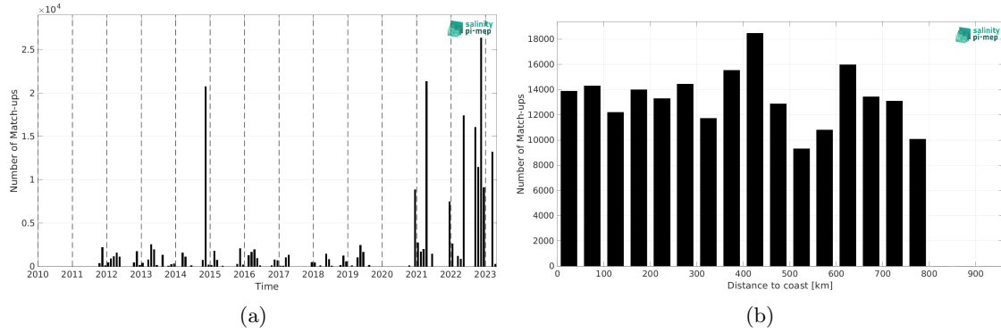
Figure 2: Number of match-ups between TSG (Polarstern) and SMAP SSS L4 OI v3 - Monthly (ESR) SSS as a function of time (a) and as function of the distance to coast (b) over the SMOS coastal zone (<800km) 60N-60S Pi-MEP region and for the full satellite product period.
