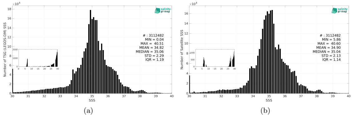
Figure 3: Histograms of SSS from TSG (LEGOS-DM) (a) and SMAP SSS L4 OI v3 - Monthly (ESR) (b) considering all match-up pairs per bins of 0.1 over the SMOS coastal zone (<800km) 60N-60S Pi-MEP region and for the full satellite product period.
