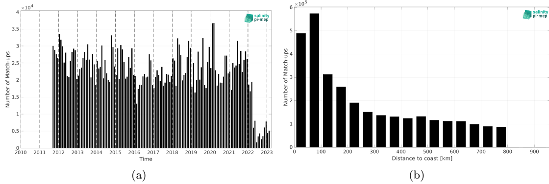
Figure 2: Number of match-ups between TSG (LEGOS-DM) and SMAP SSS L4 OI v3 - Monthly (ESR) SSS as a function of time (a) and as function of the distance to coast (b) over the SMOS coastal zone (<800km) 60N-60S Pi-MEP region and for the full satellite product period.
