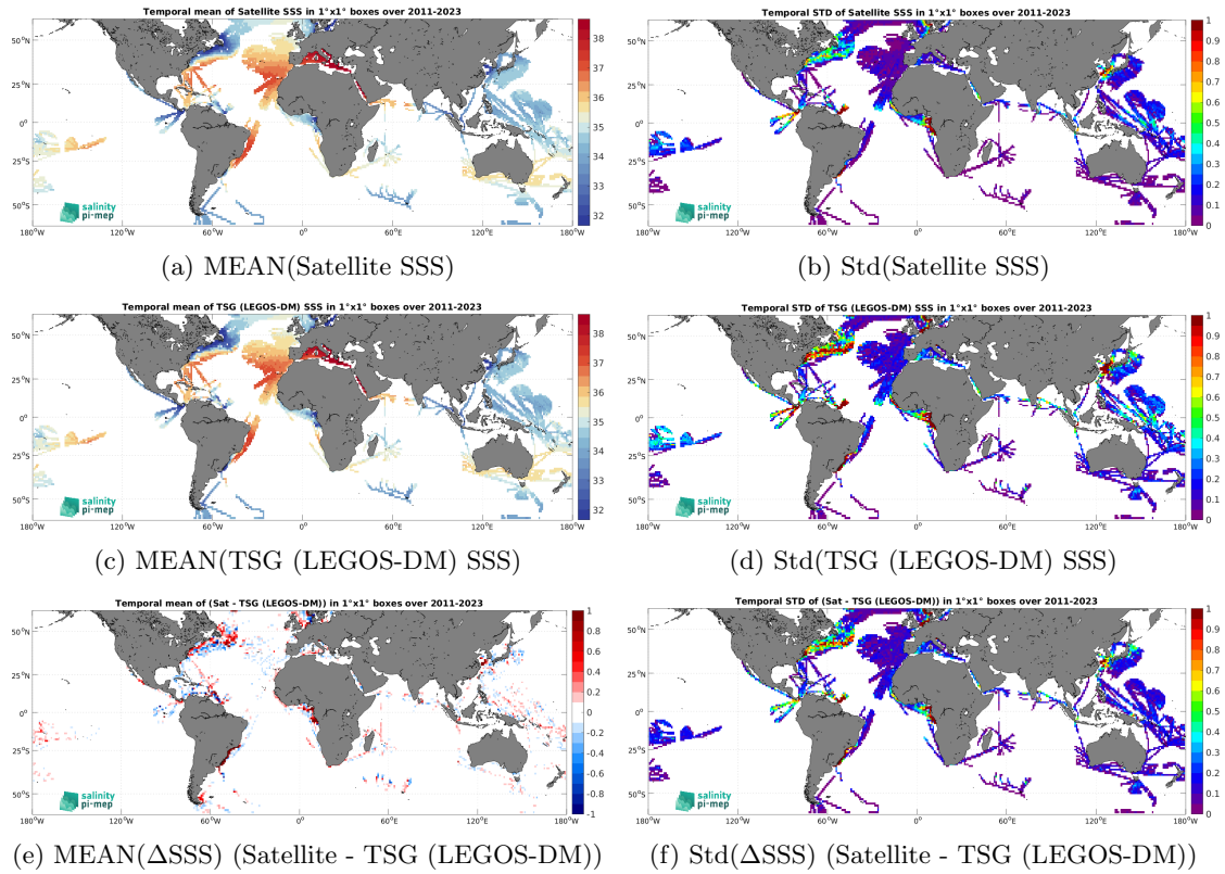
Figure 7: Temporal mean (left) and Std (right) of SSS from SMAP SSS L4 OI v3 - Monthly (ESR) (top), TSG (LEGOS-DM) (middle), and of \Delta SSS (Satellite - TSG (LEGOS-DM)). Only match-up pairs are used to generate these maps.
