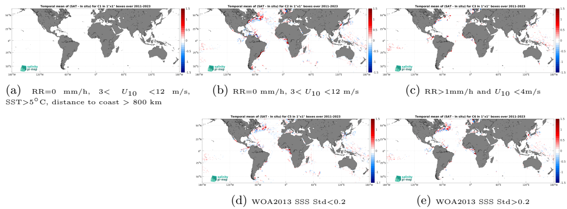
Figure 14: Temporal mean gridded over spatial boxes of size 1^\circ \times 1^\circ of \Delta\text{SSS} (SMAP SSS L4 OI v3 - Monthly (ESR) - TSG (LEGOS-DM)) for 5 different subdatasets corresponding to:RR=0 mm/h, 3 < U_{10} < 12 m/s, SST >5^\circ\text{C} , distance to coast > 800 km (a), RR=0 mm/h, 3 < U_{10} < 12 m/s (b), RR >1 mm/h and U_{10} < 4 m/s (c), WOA2013 SSS Std <0.2 (d), WOA2013 SSS Std >0.2 (e).
