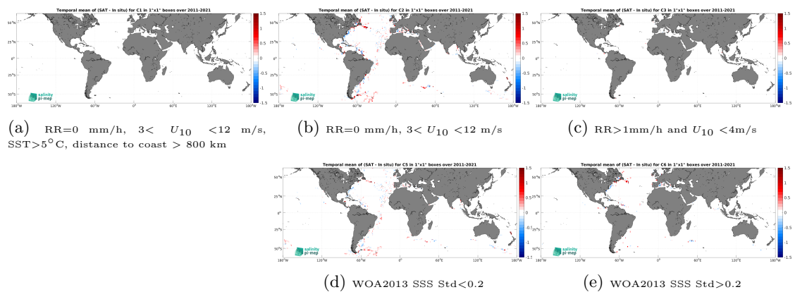
Figure 14: Temporal mean gridded over spatial boxes of size 1^\circ \times 1^\circ of \Delta SSS (SMAP SSS L4 OI v3 - Monthly (ESR) - TSG (GOSUD-Sailing-ship)) for 5 different subdatasets corresponding to:RR=0 mm/h, 3 < U_{10} < 12 m/s, SST >5^\circ C, distance to coast > 800 km (a), RR=0 mm/h, 3 < U_{10} < 12 m/s (b), RR >1 mm/h and U_{10} < 4 m/s (c), WOA2013 SSS Std <0.2 (d), WOA2013 SSS Std >0.2 (e).
