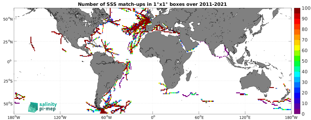
Figure 5: Number of SSS match-ups between TSG (GOSUD-Sailing-ship) SSS and the SMAP SSS L4 OI v3 - Monthly (ESR) SSS product for the SMOS coastal zone (<800km) 60N-60S Pi-MEP region over 1^{\circ} \times 1^{\circ} boxes and for the full satellite product period.
