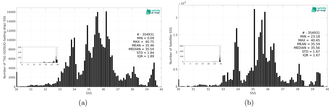
Figure 3: Histograms of SSS from TSG (GOSUD-Sailing-ship) (a) and SMAP SSS L4 OI v3 - Monthly (ESR) (b) considering all match-up pairs per bins of 0.1 over the SMOS coastal zone (<800km) 60N-60S Pi-MEP region and for the full satellite product period.
