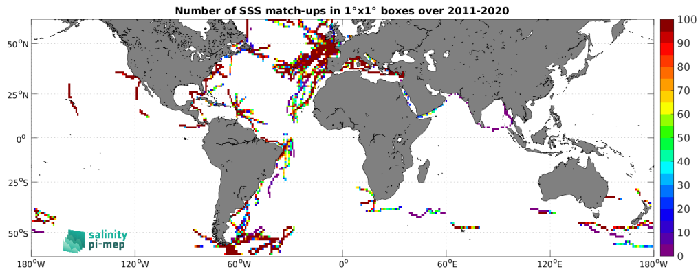
Figure 5: Number of SSS match-ups between TSG (GOSUD-Sailing-ship) SSS and the SMAP SSS L4 OI v3 - Monthly (ESR) SSS product for the SMOS coastal zone (<800km) 60N-60S Pi-MEP region over 1^\circ \times 1^\circ boxes and for the full satellite product period.
