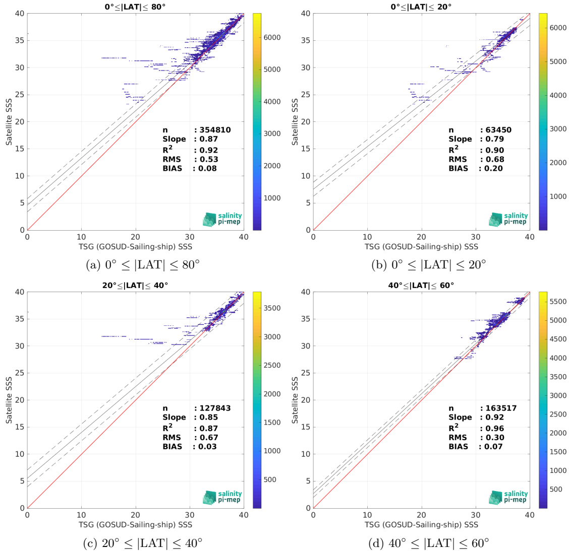
Figure 10: Contour maps of the concentration of SMAP SSS L4 OI v3 - Monthly (ESR) SSS (y-axis) versus TSG (GOSUD-Sailing-ship) SSS (x-axis) at match-up pairs for different latitude bands. For each plot, the red line shows x=y . The black thin and dashed lines indicate a linear fit through the data cloud and the \pm 95\% confidence levels, respectively. The number match-up pairs n , the slope and R^2 coefficient of the linear fit, the root mean square (RMS) and the mean bias between satellite and in situ data are indicated for each latitude band in each plots.
