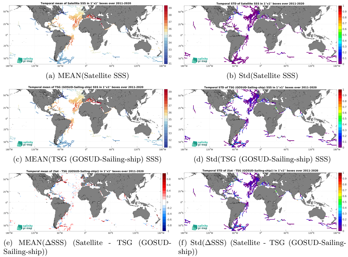
Figure 7: Temporal mean (left) and Std (right) of SSS from SMAP SSS L4 OI v3 - Monthly (ESR) (top), TSG (GOSUD-Sailing-ship) (middle), and of \Delta SSS (Satellite - TSG (GOSUD-Sailing-ship)). Only match-up pairs are used to generate these maps.
