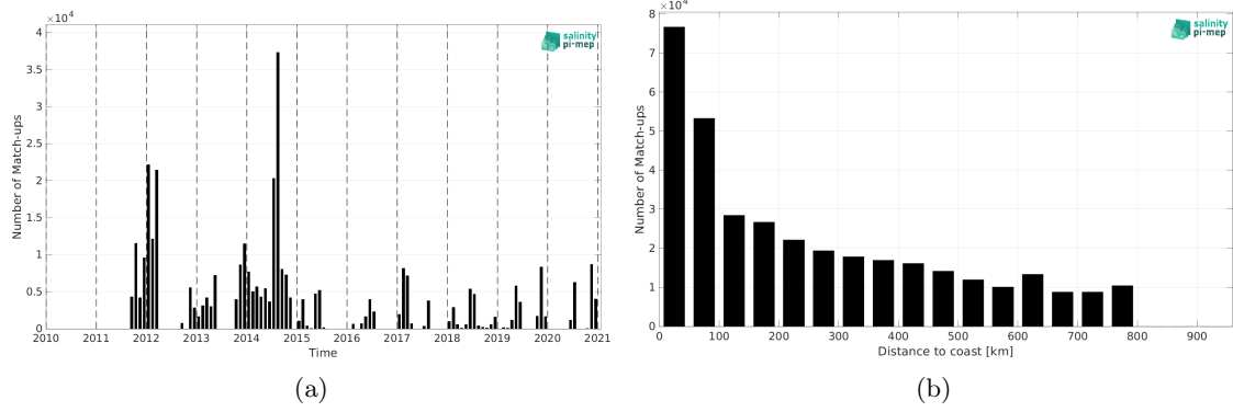
Figure 2: Number of match-ups between TSG (GOSUD-Sailing-ship) and SMAP SSS L4 OI v3 - Monthly (ESR) SSS as a function of time (a) and as function of the distance to coast (b) over the SMOS coastal zone (<800km) 60N-60S Pi-MEP region and for the full satellite product period.
