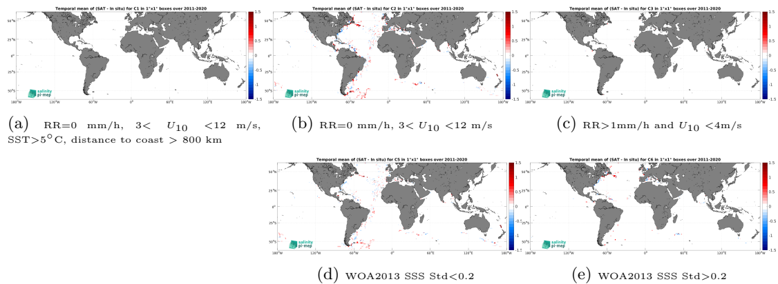
Figure 14: Temporal mean gridded over spatial boxes of size 1^\circ \times 1^\circ of \Delta\text{SSS} (SMAP SSS L4 OI v3 - Monthly (ESR) - TSG (GOSUD-Sailing-ship)) for 5 different subdatasets corresponding to:RR=0 mm/h, 3 < U_{10} < 12 m/s, SST>5°C, distance to coast > 800 km (a), RR=0 mm/h, 3 < U_{10} < 12 m/s (b), RR>1mm/h and U_{10} < 4 m/s (c), WOA2013 SSS Std<0.2 (d), WOA2013 SSS Std>0.2 (e).
