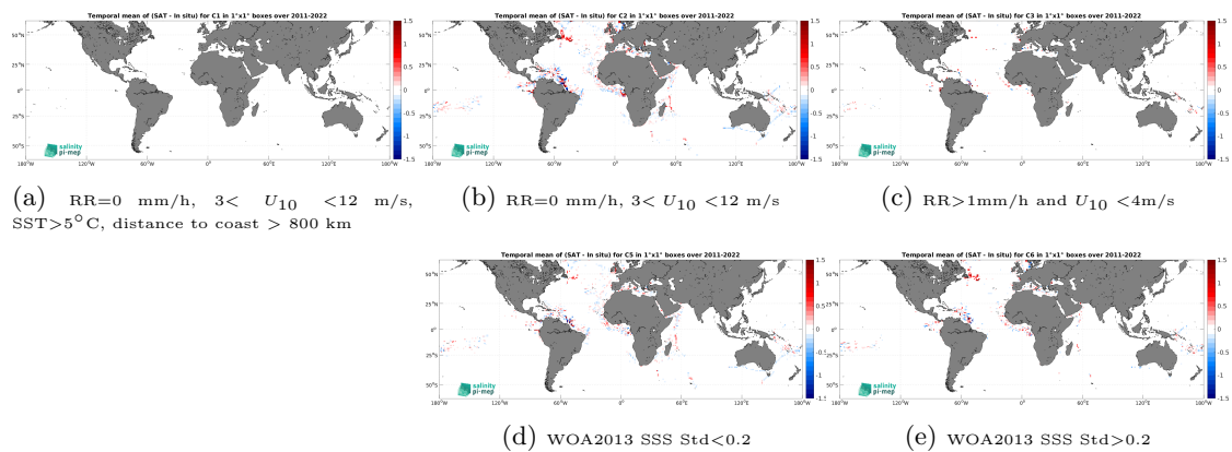
Figure 14: Temporal mean gridded over spatial boxes of size 1^\circ \times 1^\circ of \Delta\text{SSS} (SMAP SSS L4 OI v3 - Monthly (ESR) - TSG (GOSUD-Research-vessel)) for 5 different subdatasets corresponding to:RR=0 mm/h, 3 < U_{10} < 12 m/s, SST >5^\circ\text{C} , distance to coast > 800 km (a), RR=0 mm/h, 3 < U_{10} < 12 m/s (b), RR >1 mm/h and U_{10} < 4 m/s (c), WOA2013 SSS Std <0.2 (d), WOA2013 SSS Std >0.2 (e).
