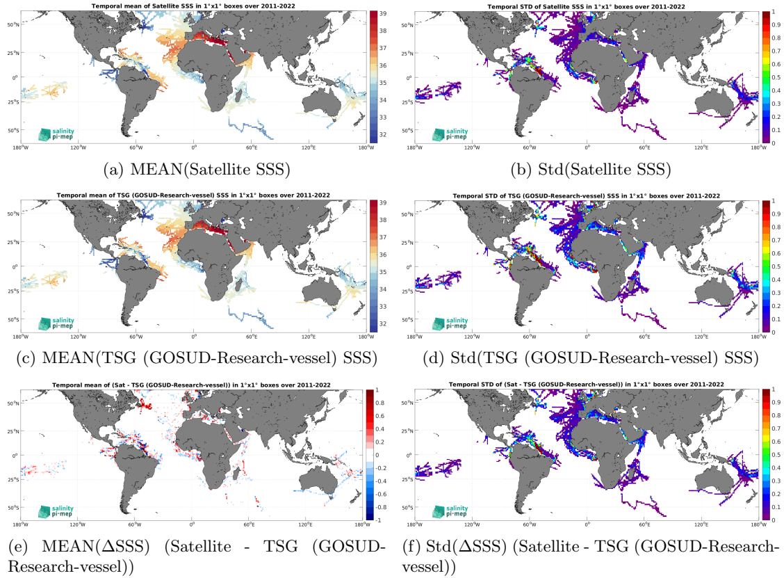
Figure 7: Temporal mean (left) and Std (right) of SSS from SMAP SSS L4 OI v3 - Monthly (ESR) (top), TSG (GOSUD-Research-vessel) (middle), and of \Delta SSS (Satellite - TSG (GOSUD-Research-vessel)). Only match-up pairs are used to generate these maps.
