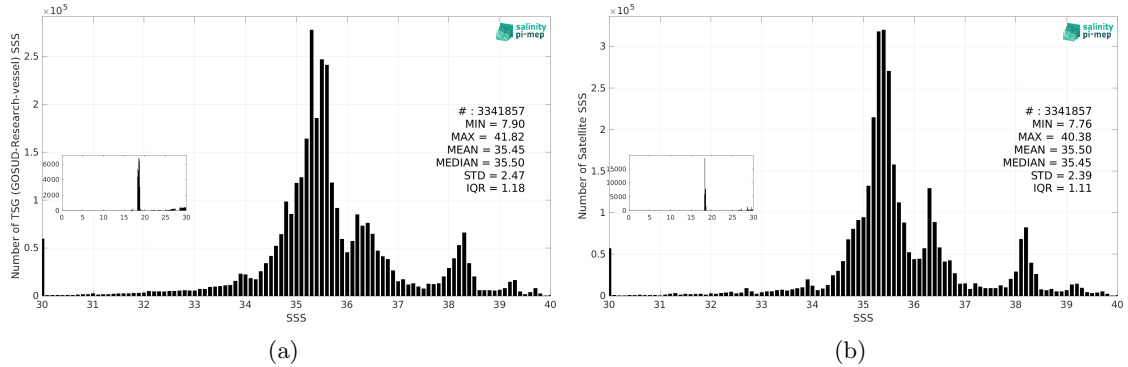
Figure 3: Histograms of SSS from TSG (GOSUD-Research-vessel) (a) and SMAP SSS L4 OI v3 - Monthly (ESR) (b) considering all match-up pairs per bins of 0.1 over the SMOS coastal zone (<800km) 60N-60S Pi-MEP region and for the full satellite product period.
