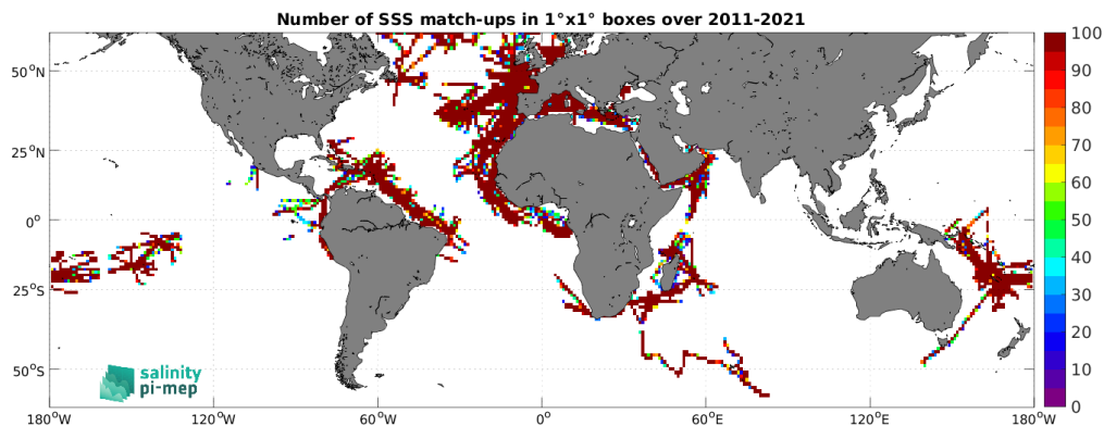
Figure 5: Number of SSS match-ups between TSG (GOSUD-Research-vessel) SSS and the SMAP SSS L4 OI v3 - Monthly (ESR) SSS product for the SMOS coastal zone ( <800\text{km} ) 60\text{N} - 60\text{S} Pi-MEP region over 1^\circ \times 1^\circ boxes and for the full satellite product period.
