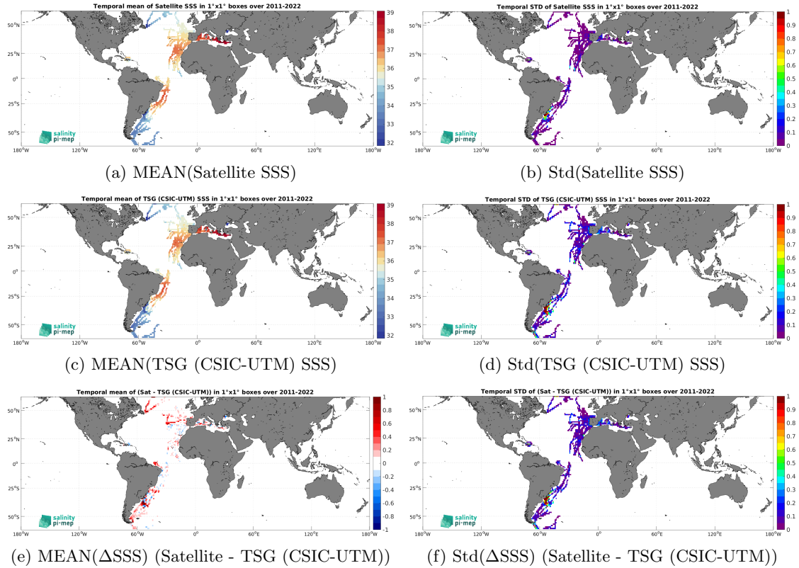
Figure 7: Temporal mean (left) and Std (right) of SSS from SMAP SSS L4 OI v3 - Monthly (ESR) (top), TSG (CSIC-UTM) (middle), and of \Delta SSS (Satellite - TSG (CSIC-UTM)). Only match-up pairs are used to generate these maps.
