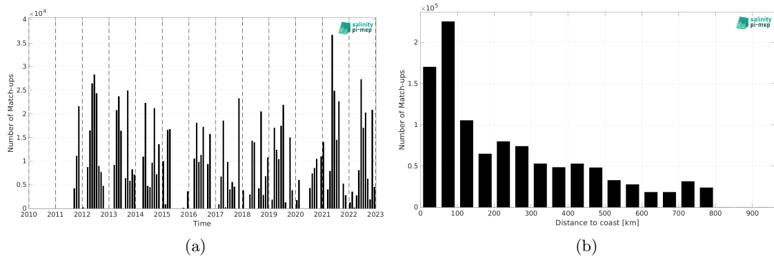
Figure 2: Number of match-ups between TSG (CSIC-UTM) and SMAP SSS L4 OI v3 - Monthly (ESR) SSS as a function of time (a) and as function of the distance to coast (b) over the SMOS coastal zone (<800km) 60N-60S Pi-MEP region and for the full satellite product period.
