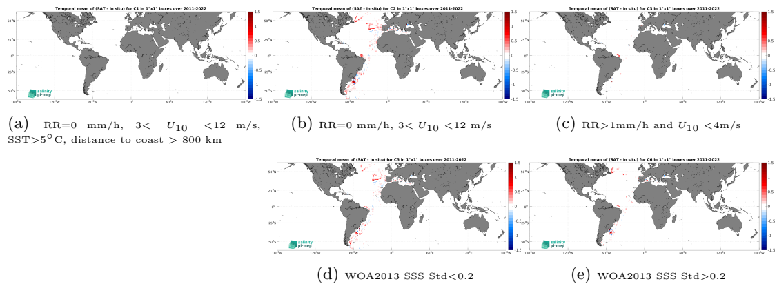
Figure 14: Temporal mean gridded over spatial boxes of size 1^\circ \times 1^\circ of \Delta\text{SSS} (SMAP SSS L4 OI v3 - Monthly (ESR) - TSG (CSIC-UTM)) for 5 different subdatasets corresponding to:RR=0 mm/h, 3 < U_{10} < 12 m/s, SST >5^\circ\text{C} , distance to coast > 800 km (a), RR=0 mm/h, 3 < U_{10} < 12 m/s (b), RR >1 mm/h and U_{10} < 4 m/s (c), WOA2013 SSS Std <0.2 (d), WOA2013 SSS Std >0.2 (e).
