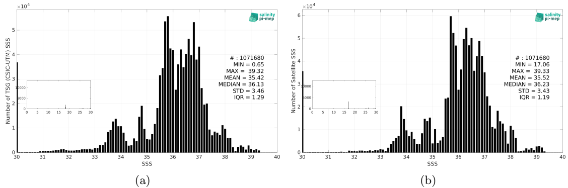
Figure 3: Histograms of SSS from TSG (CSIC-UTM) (a) and SMAP SSS L4 OI v3 - Monthly (ESR) (b) considering all match-up pairs per bins of 0.1 over the SMOS coastal zone (<800km) 60N-60S Pi-MEP region and for the full satellite product period.
