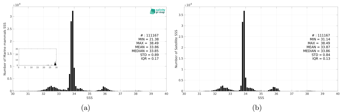
Figure 3: Histograms of SSS from Marine mammals (a) and SMAP SSS L4 OI v3 - Monthly (ESR) (b) considering all match-up pairs per bins of 0.1 over the SMOS coastal zone (<800km) 60N-60S Pi-MEP region and for the full satellite product period.
