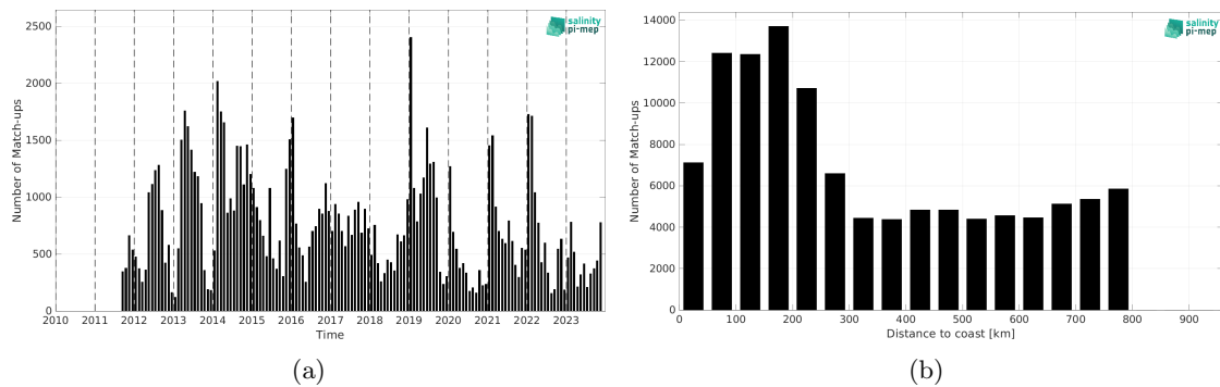
Figure 2: Number of match-ups between Marine mammals and SMAP SSS L4 OI v3 - Monthly (ESR) SSS as a function of time (a) and as function of the distance to coast (b) over the SMOS coastal zone (<800km) 60N-60S Pi-MEP region and for the full satellite product period.
