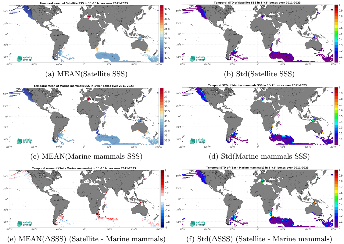
Figure 7: Temporal mean (left) and Std (right) of SSS from SMAP SSS L4 OI v3 - Monthly (ESR) (top), Marine mammals (middle), and of \Delta SSS (Satellite - Marine mammals). Only match-up pairs are used to generate these maps.
