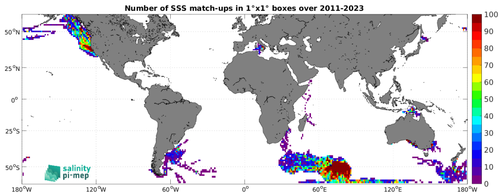
Figure 5: Number of SSS match-ups between Marine mammals SSS and the SMAP SSS L4 OI v3 - Monthly (ESR) SSS product for the SMOS coastal zone (<800km) 60N-60S Pi-MEP region over 1^\circ \times 1^\circ boxes and for the full satellite product period.
