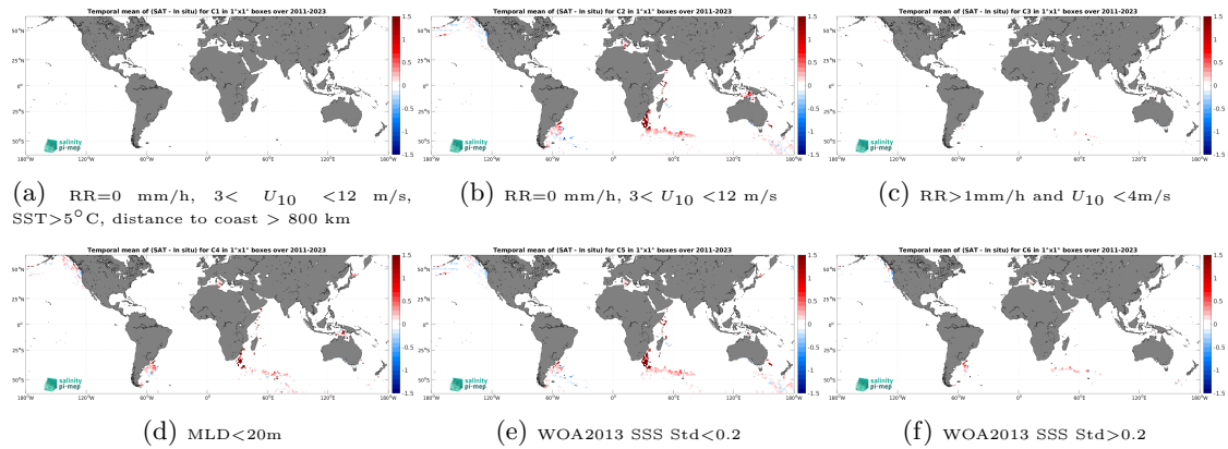
Figure 14: Temporal mean gridded over spatial boxes of size 1^\circ \times 1^\circ of \Delta SSS (SMAP SSS L4 OI v3 - Monthly (ESR) - Marine mammals) for 6 different subdatasets corresponding to:RR=0 mm/h, 3 < U_{10} < 12 m/s, SST >5^\circ C, distance to coast > 800 km (a), RR=0 mm/h, 3 < U_{10} < 12 m/s (b), RR >1 mm/h and U_{10} < 4 m/s (c),MLD <20 m (d),WOA2013 SSS Std <0.2 (e),WOA2013 SSS Std >0.2 (f).
