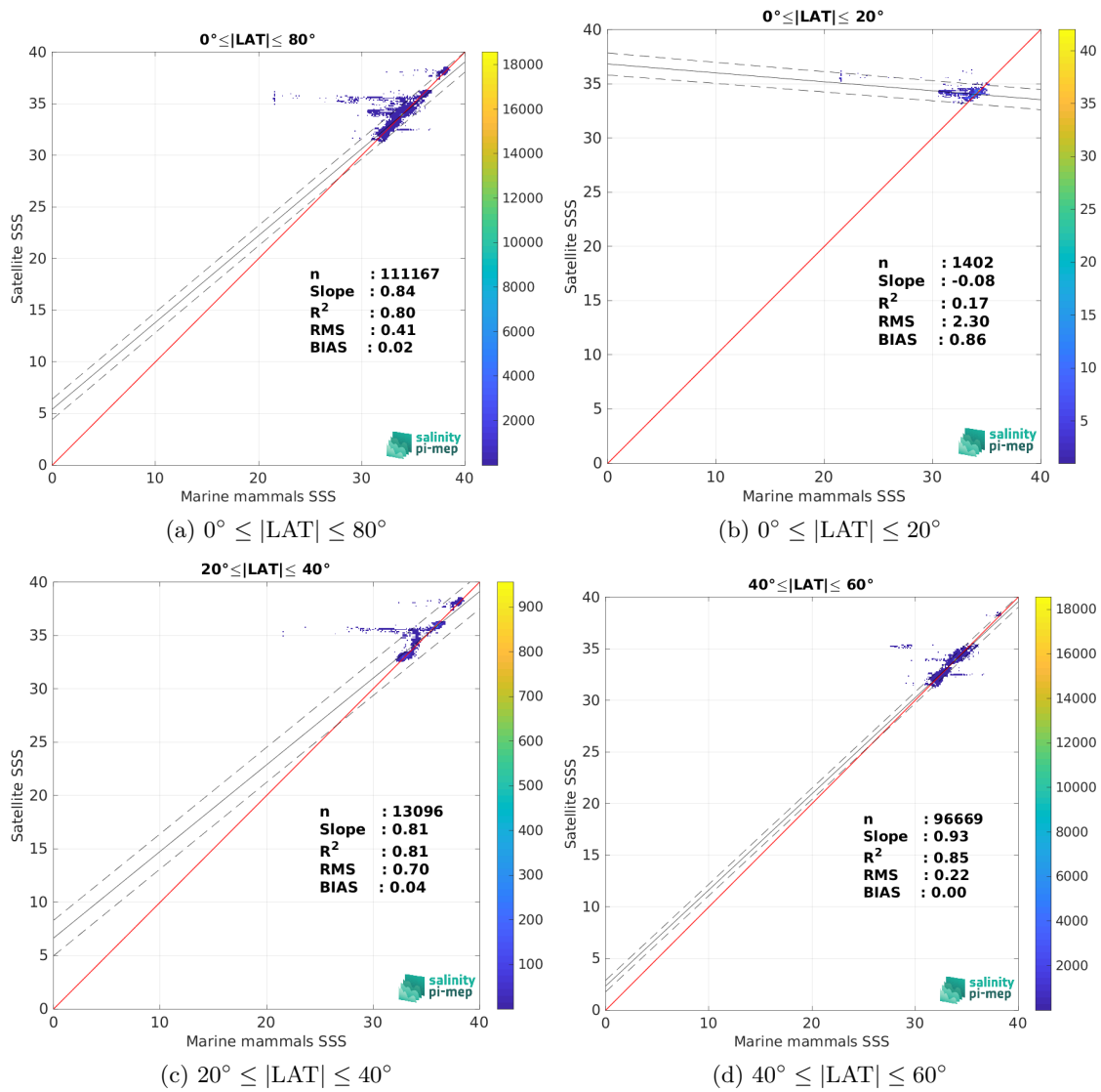
Figure 10: Contour maps of the concentration of SMAP SSS L4 OI v3 - Monthly (ESR) SSS (y-axis) versus Marine mammals SSS (x-axis) at match-up pairs for different latitude bands. For each plot, the red line shows x=y . The black thin and dashed lines indicate a linear fit through the data cloud and the \pm 95\% confidence levels, respectively. The number match-up pairs n , the slope and R^2 coefficient of the linear fit, the root mean square (RMS) and the mean bias between satellite and in situ data are indicated for each latitude band in each plots.
