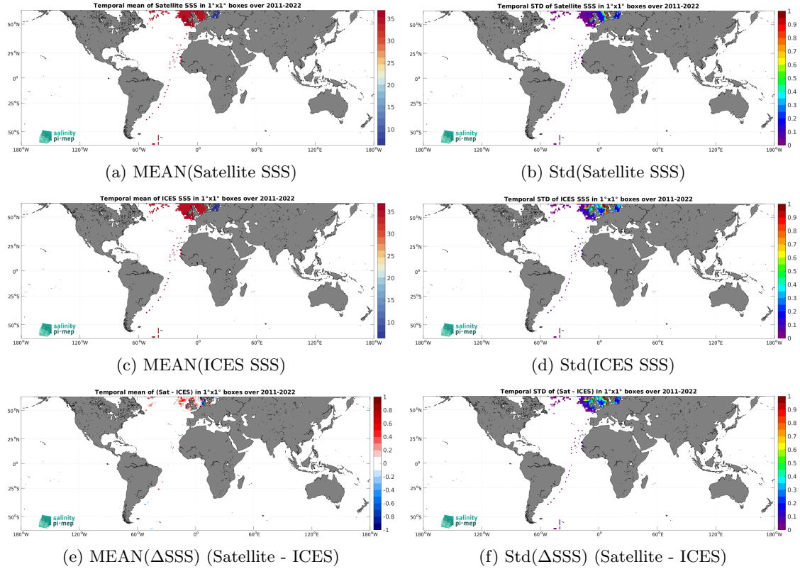
Figure 7: Temporal mean (left) and Std (right) of SSS from SMAP SSS L4 OI v3 - Monthly (ESR) (top), ICES (middle), and of \Delta SSS (Satellite - ICES). Only match-up pairs are used to generate these maps.
