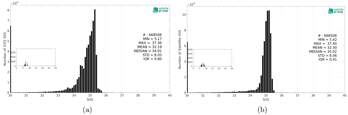
Figure 3: Histograms of SSS from ICES (a) and SMAP SSS L4 OI v3 - Monthly (ESR) (b) considering all match-up pairs per bins of 0.1 over the SMOS coastal zone (<800km) 60N-60S Pi-MEP region and for the full satellite product period.
