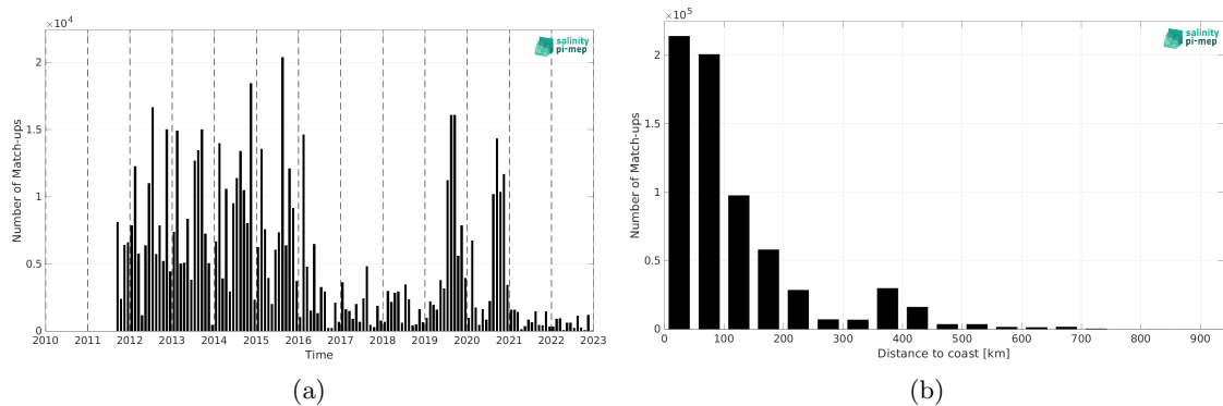
Figure 2: Number of match-ups between ICES and SMAP SSS L4 OI v3 - Monthly (ESR) SSS as a function of time (a) and as function of the distance to coast (b) over the SMOS coastal zone (<800km) 60N-60S Pi-MEP region and for the full satellite product period.
