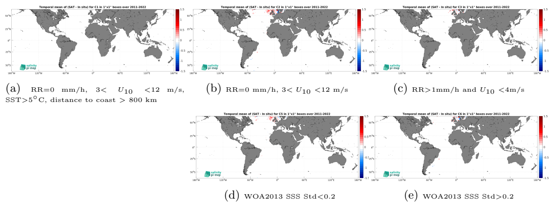
Figure 14: Temporal mean gridded over spatial boxes of size 1^\circ \times 1^\circ of \Delta\text{SSS} (SMAP SSS L4 OI v3 - Monthly (ESR) - ICES) for 5 different subdatasets corresponding to:RR=0 mm/h, 3 < U_{10} < 12 m/s, SST >5^\circ\text{C} , distance to coast > 800 km (a), RR=0 mm/h, 3 < U_{10} < 12 m/s (b), RR >1 mm/h and U_{10} < 4 m/s (c), WOA2013 SSS Std <0.2 (d), WOA2013 SSS Std >0.2 (e).
